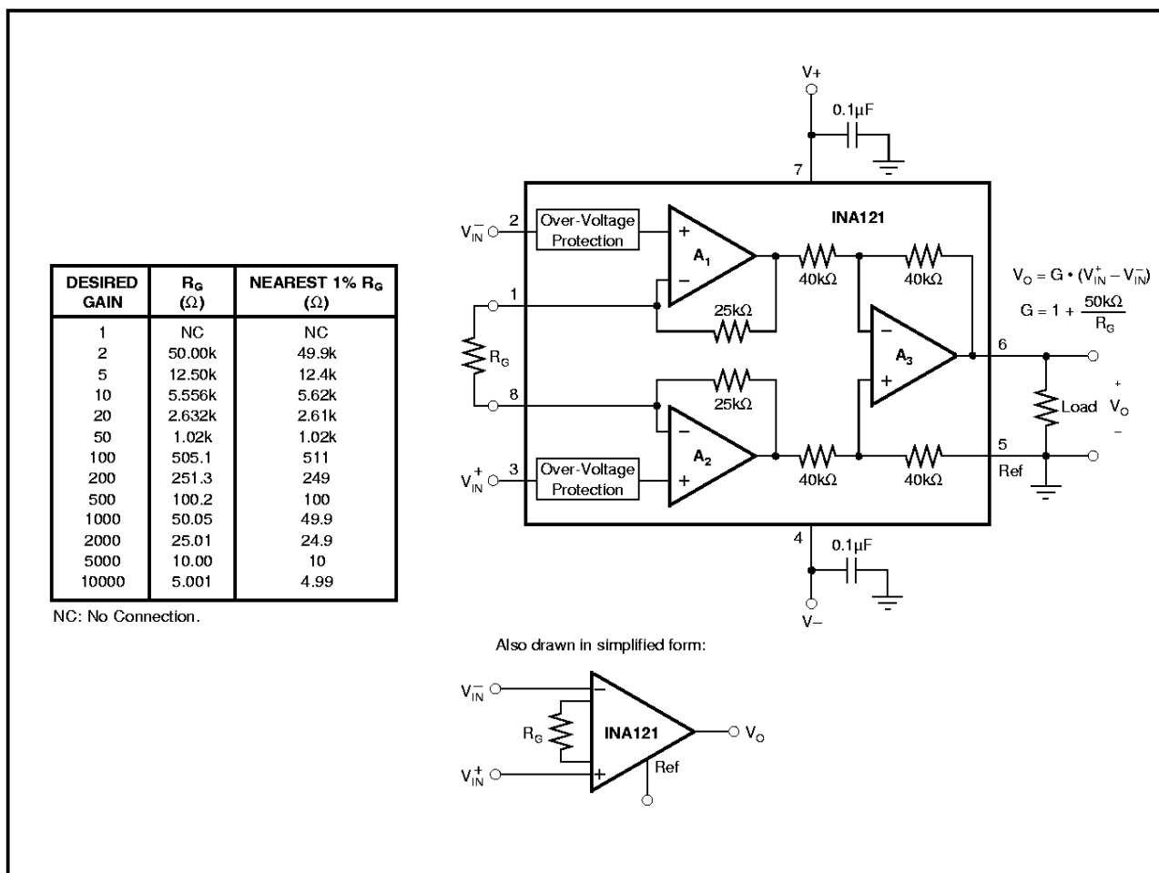
FIGURE 1. Basic Connections.
