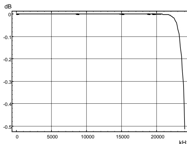
Fig. 2–7: 1 to 4 Oversampling filter, pass-band
