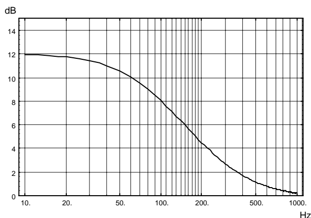
Fig. 2–6: Bass boost
