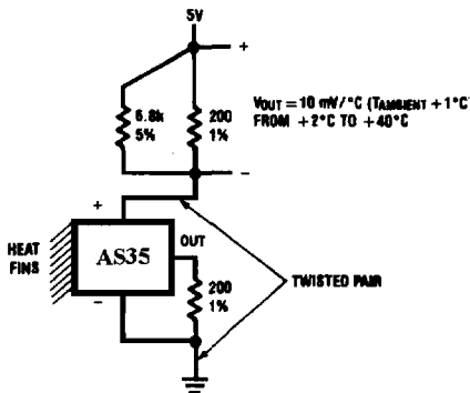
Two-Wire Remote Temperature Sensor (Grounded Sensor)
