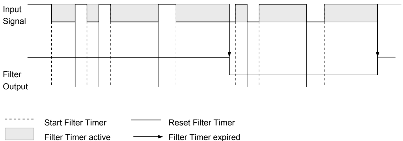
Figure 12: Principle of input filtering
