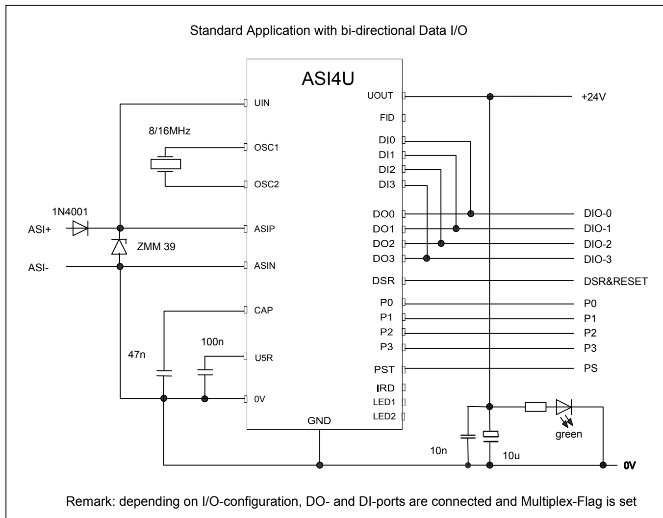
Figure 20: Standard Application circuit with bi-directional Data I/O
