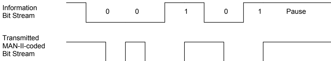
Figure 19: Manchester-II-Modulation principle
