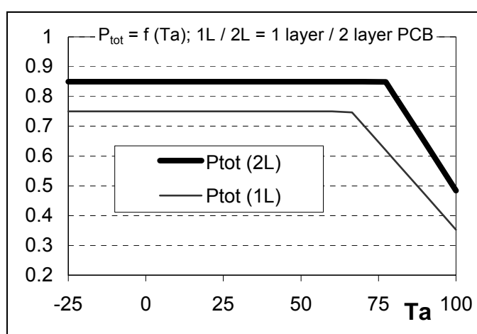
Figure 1: P_{tot} = f(\theta_a)
