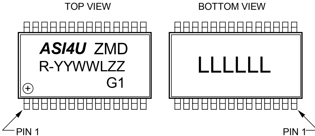
Figure 27: Package Marking
