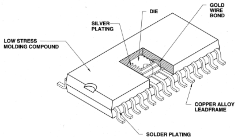
Figure 23: SOP Package
