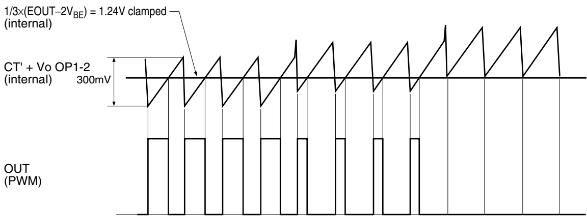
Timing Chart 7 (Current Limiting)
