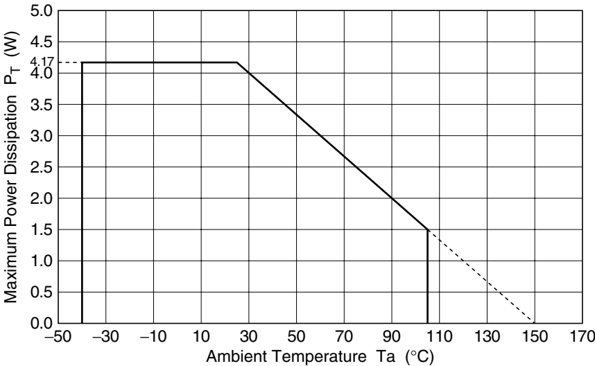
Figure 1 Derating Curve
