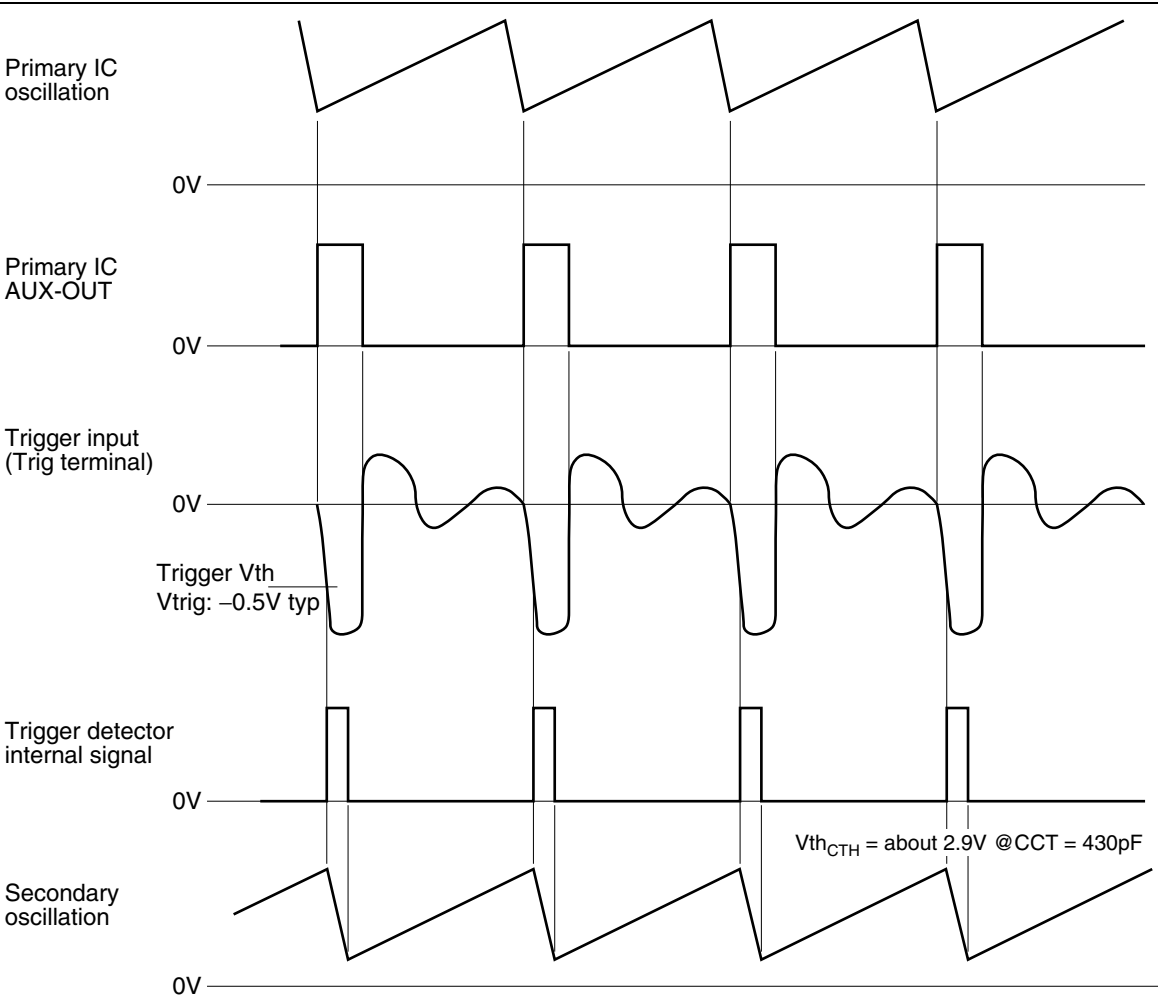
Timing Chart 5 (External Trigger Control)
