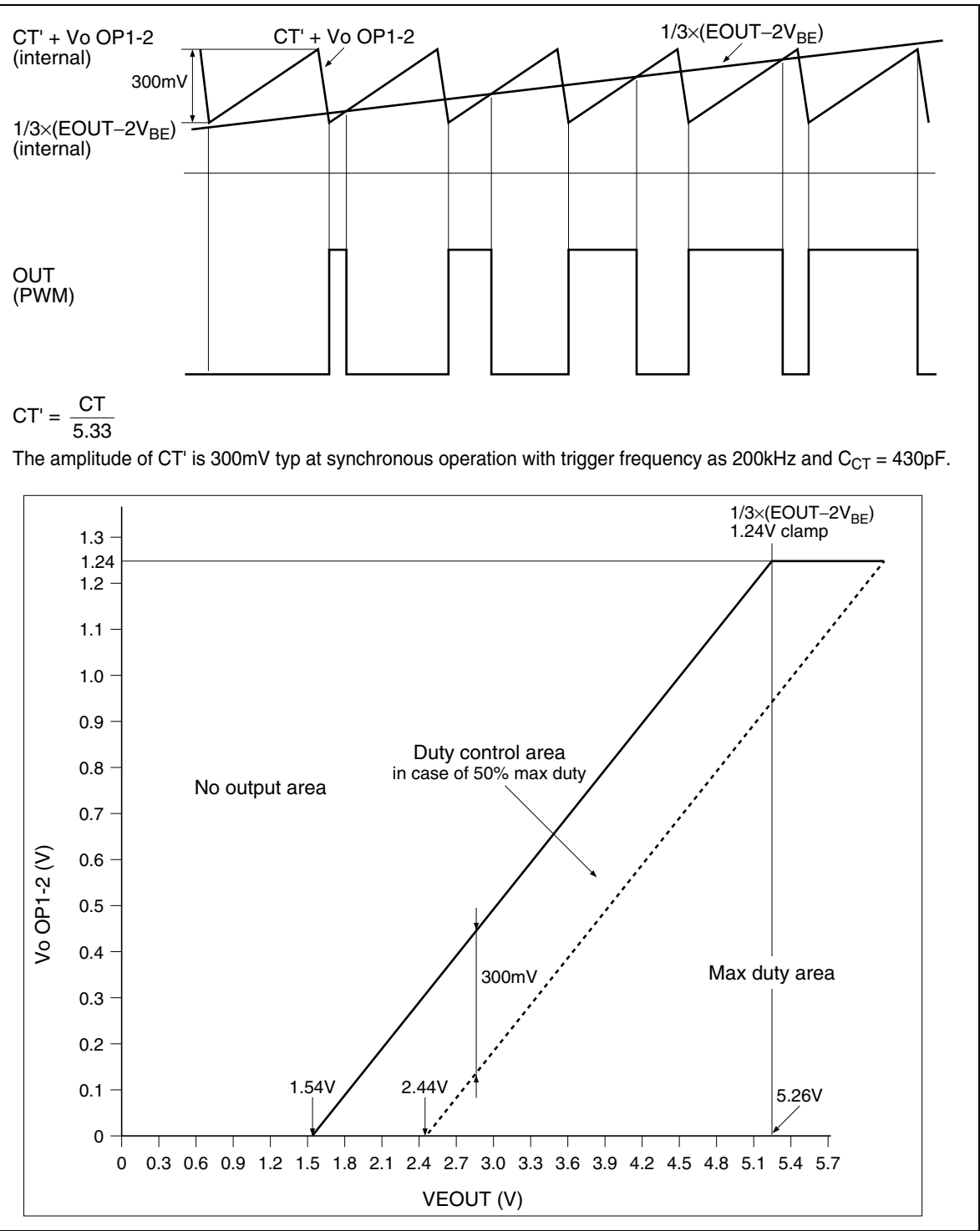
Timing Chart 6 (Duty Control)
