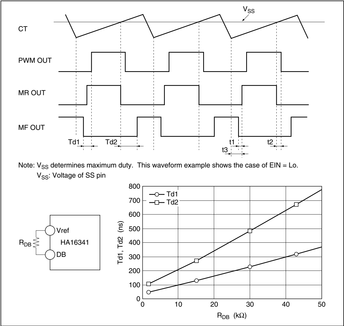
Timing Chart 3 (Dead Band Control)
