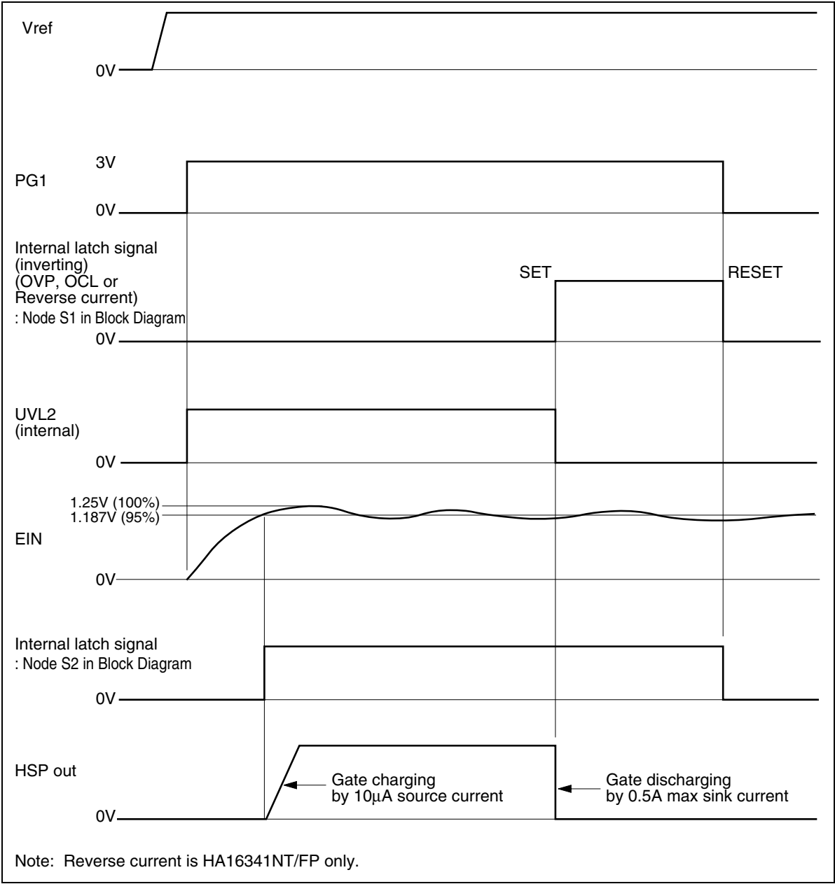
Timing Chart 2 (Hot Swap)
