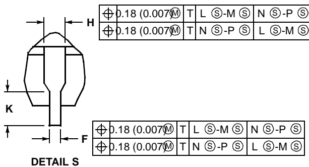
DETAIL S
