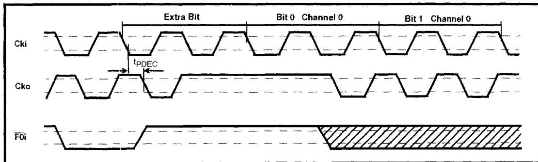
Figure 10 - Cko Timing with Extra Bit Insertion Mode
