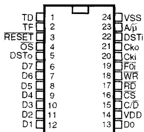
Figure 2 - Pin Connections
