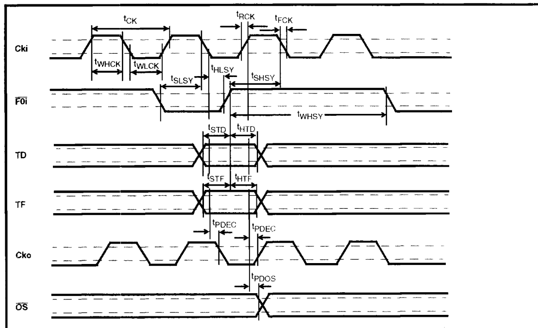
Figure 5 - Clock Timing
