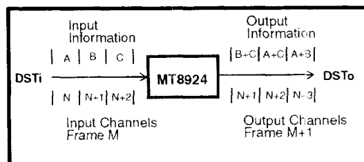
Figure 4 - Input/Output Channel Relationship
