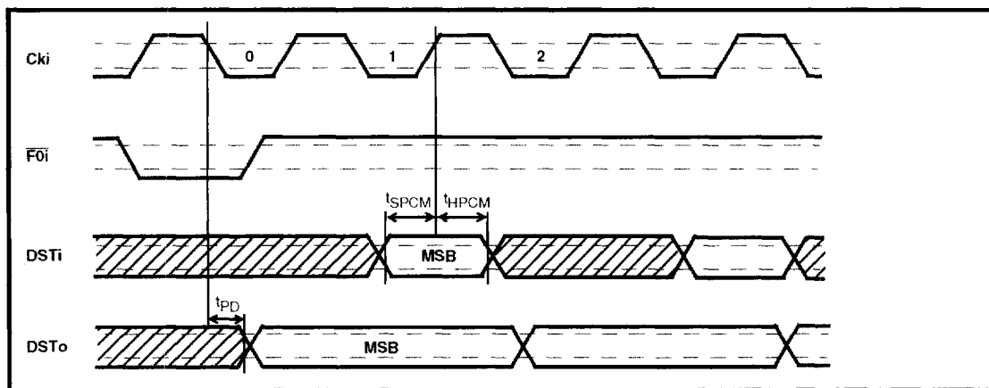
Figure 6 - PCM Timing
