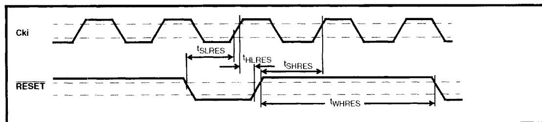
Figure 7 - Reset Timing
