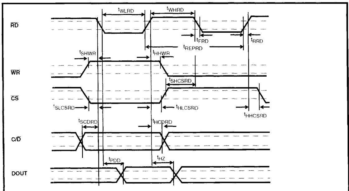
Figure 9 - Read Timing Characteristics
