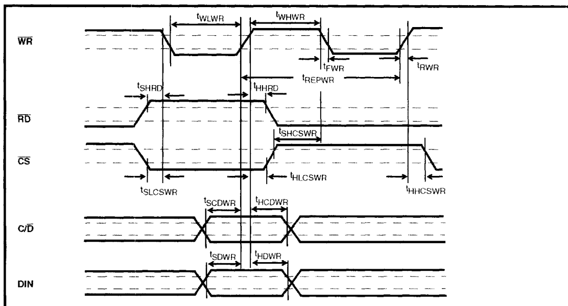
Figure 8 - Write Timing Characteristics
