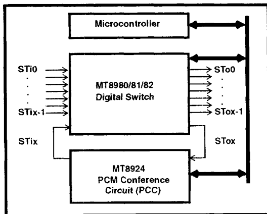
Figure 3 - Typical Conference Connection
