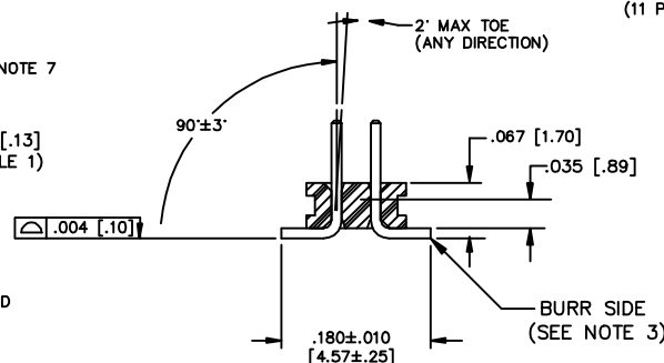
SECT "A-A" (ROTATED 90°)
