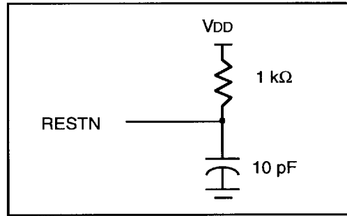
Figure 17. RESTN Test Load Circuit
