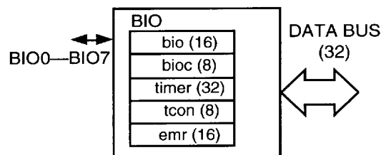
Figure 5. Timer/Bit I/O (BIO)
