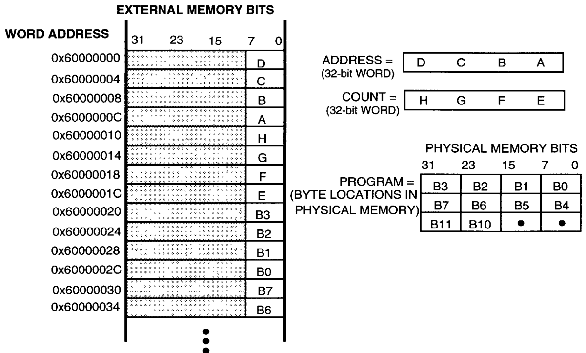
Figure 7. EPROM Data Organization (DSP3207 Begins Execution in Big-Endian Mode)
