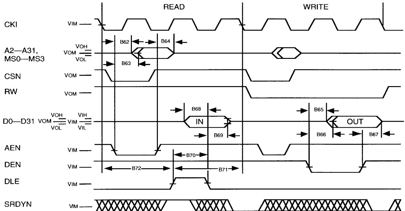
Figure 13. Asynchronous Bus Interface Timing
