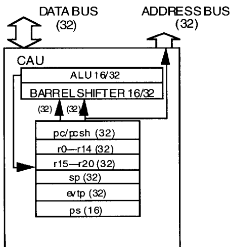
Figure 3. Control Arithmetic Unit (CAU)
