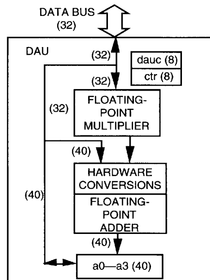
Figure 4. Data Arithmetic Unit (DAU)
