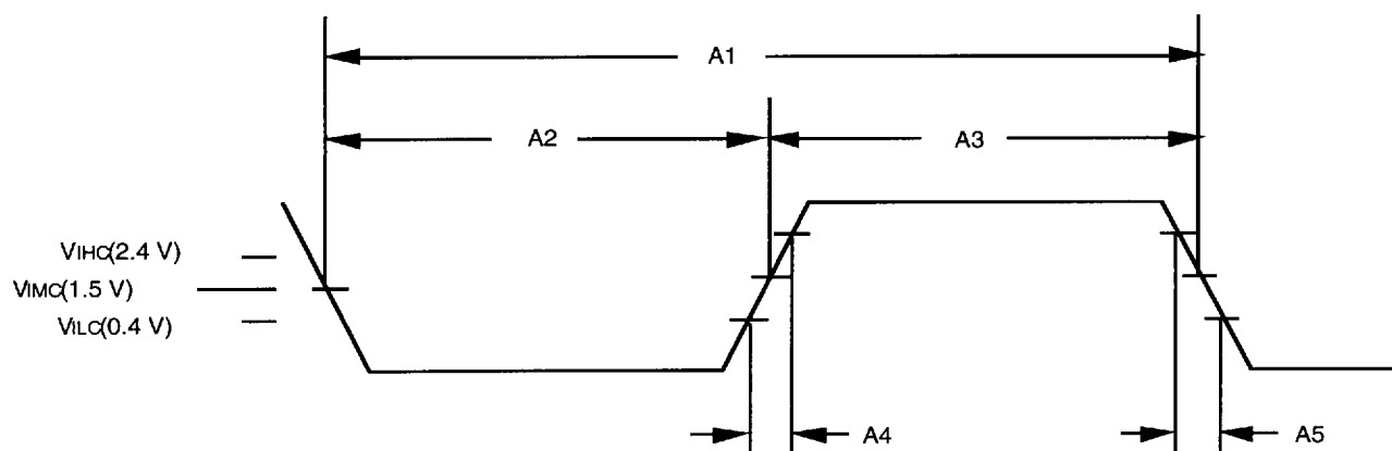
Figure 11. CKI Timing Specifications
