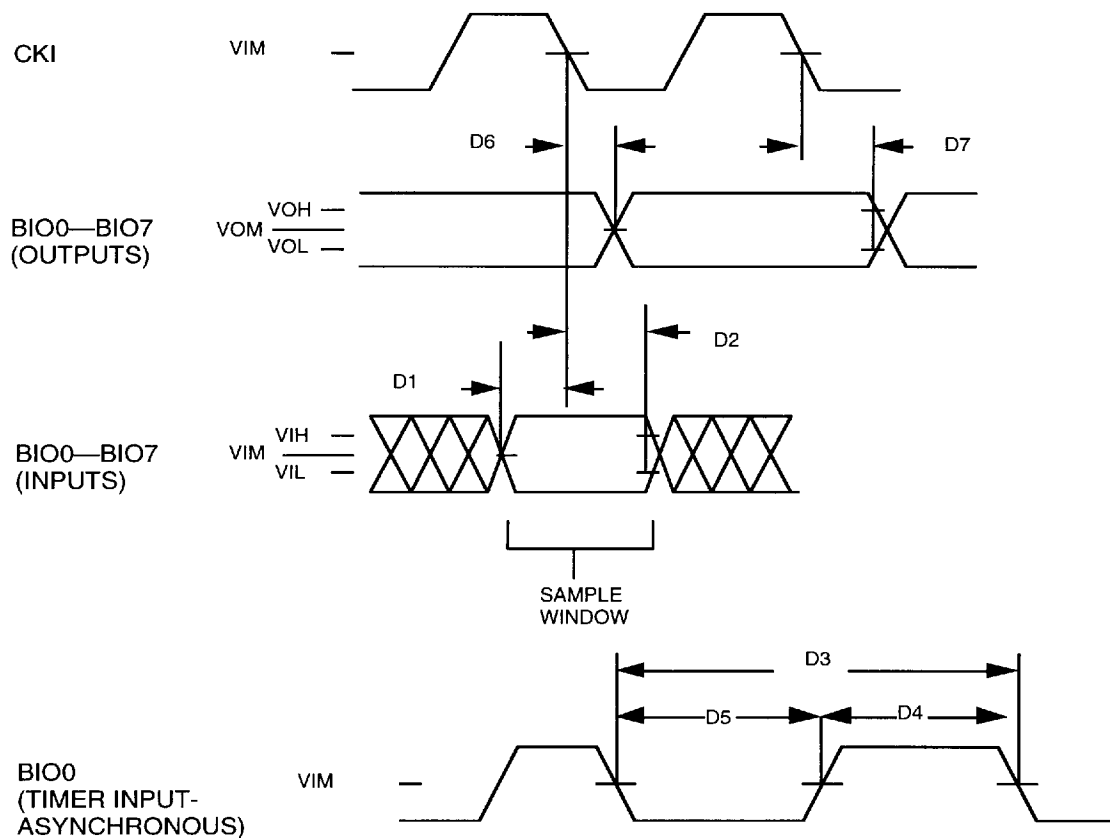
Figure 15. Bit I/O Timing
