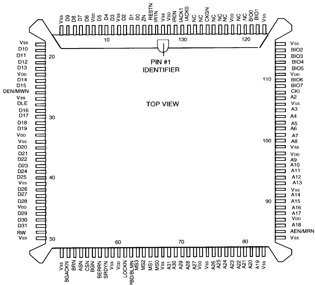
Figure 8. 132-Pin PQFP Pin Diagram
