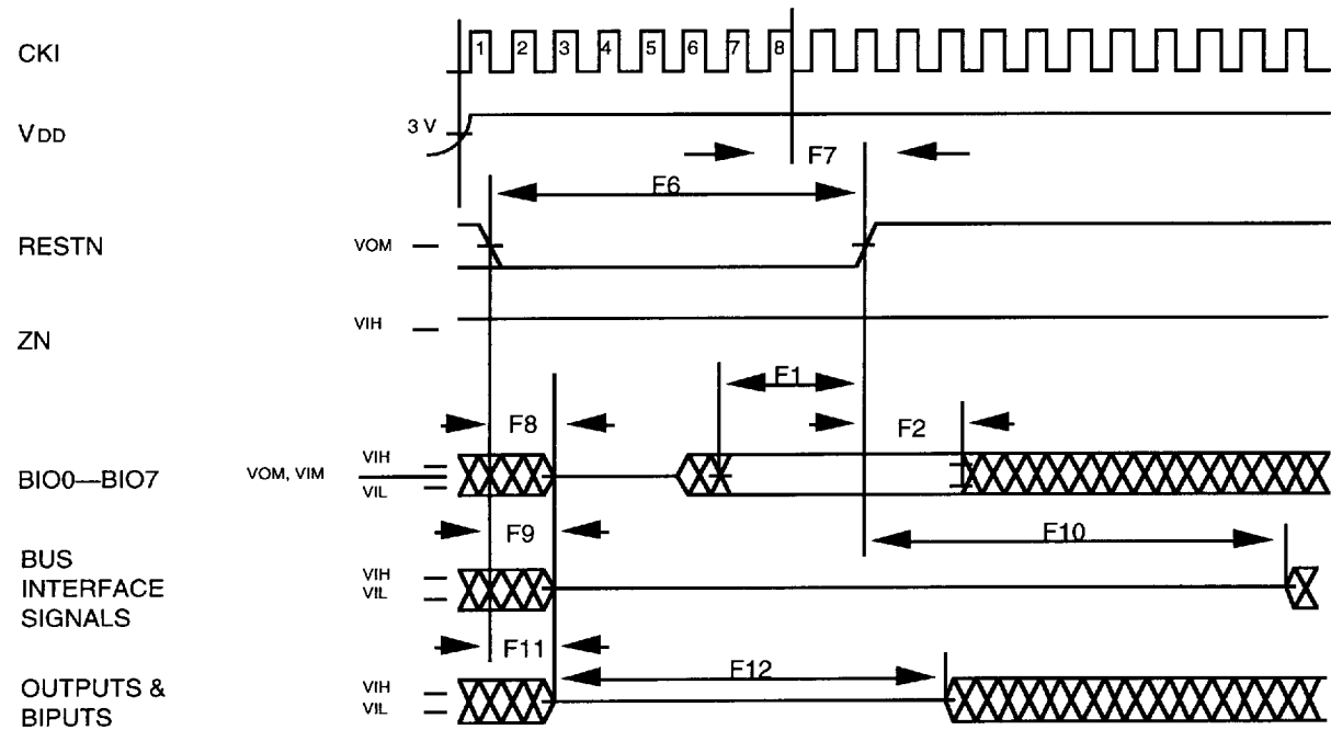
Figure 18. Power-On Reset Timing
