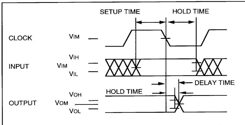
Figure 10. ac Testing Input/Output Waveform
