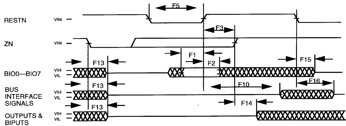
Figure 19. Externally Controlled Reset and ZN Timing
