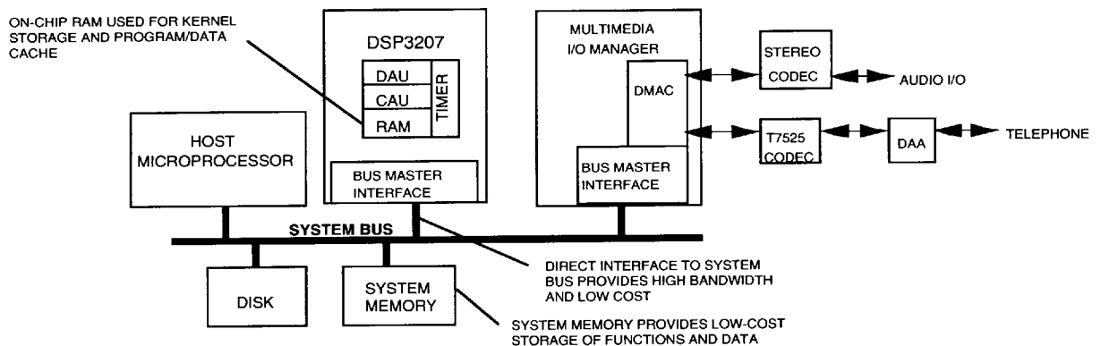
Figure 2. Typical DSP3207 PC/Workstation Motherboard Configuration
