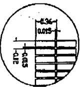
DETAIL A
