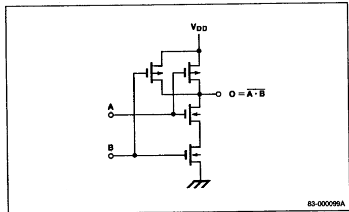
Figure 2. Cell Configured as a Two-Input NAND Gate
