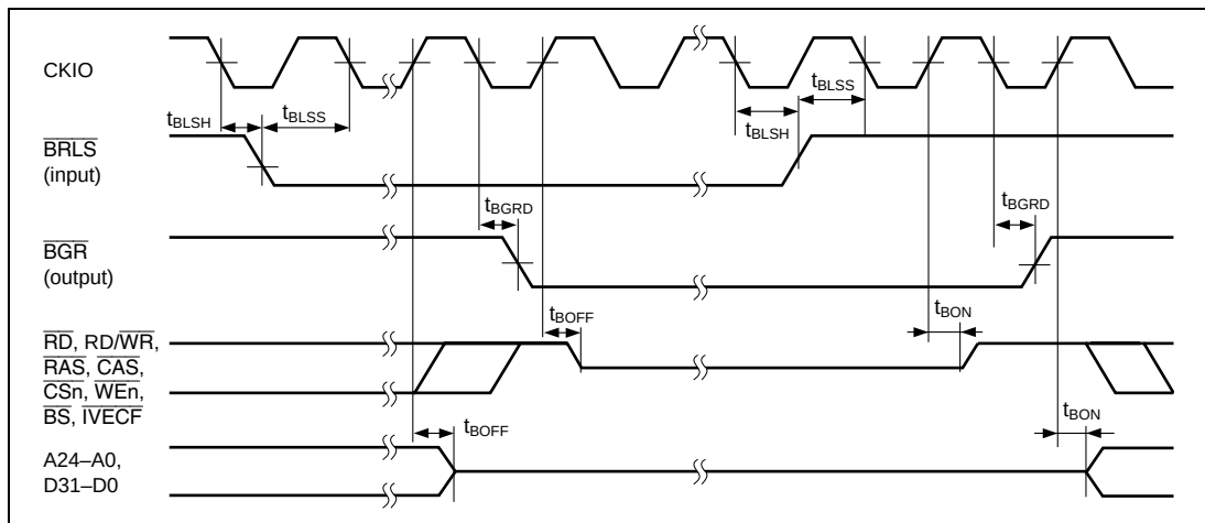
Figure 21.11 Bus Release Timing
