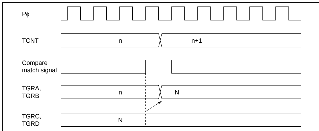
Figure 16.36 Buffer Operation Timing (Compare Match)
