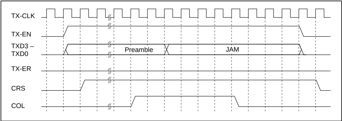
Figure 9.4 (b) MII Frame Transmit Timing (Collision)
