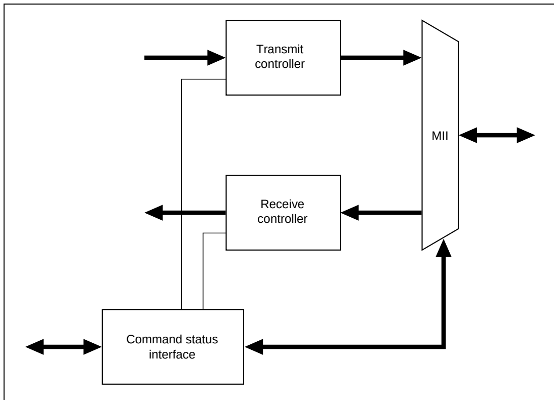
Figure 9.1 Configuration of Ethernet Controller (EtherC)
