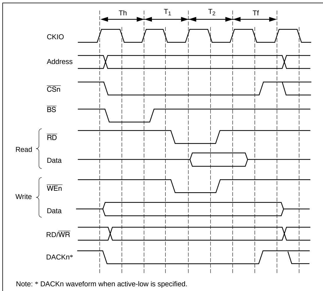
Figure 7.16 \overline{\text{CS}} Assertion Period Extension Function
