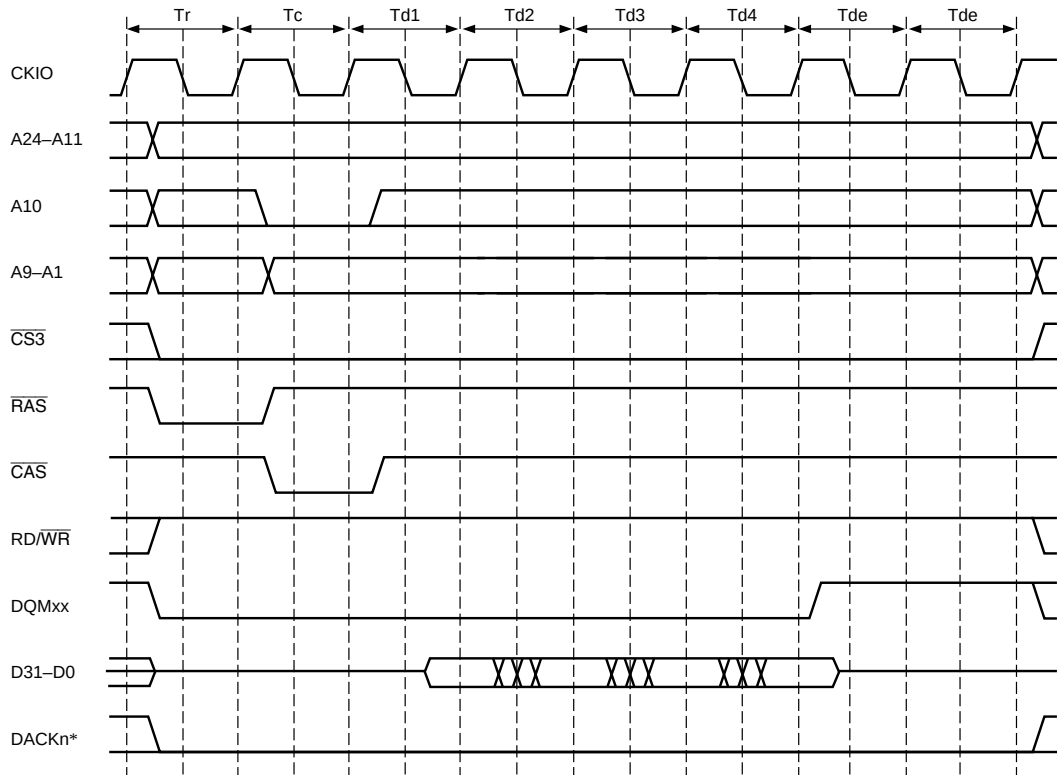
Figure 7.24 (b) Burst Read Timing (No Precharge) I\phi:E\phi = 1:1
