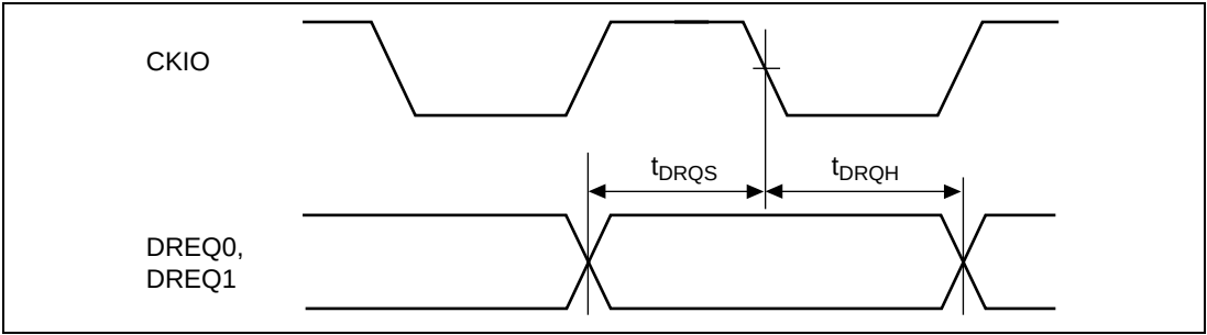
Figure 21.48 DREQ0, DREQ1 Input Timing
