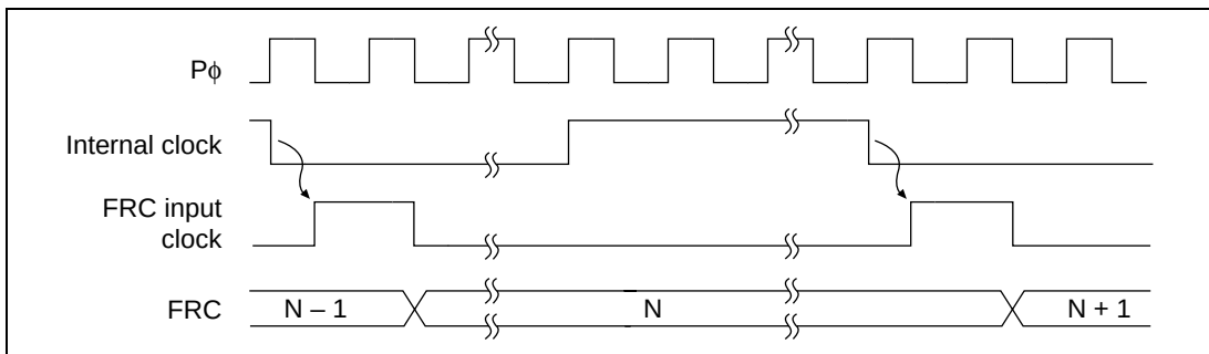
Figure 12.4 Count Timing (Internal Clock Operation)
