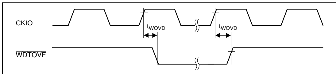
Figure 21.59 Watchdog Timer Output Timing ( t_{E_{cyc}}:t_{P_{cyc}} = 1:1 )
