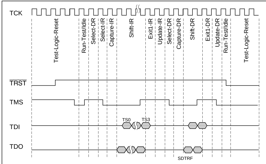
Figure 17.4 Data Input/Output Timing Chart (2)
