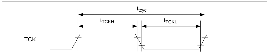
Figure 21.65 H-UDI Clock Timing
