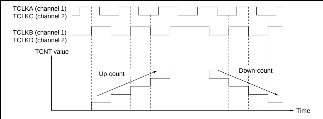
Figure 16.29 Example of Phase Counting Mode 4 Operation
