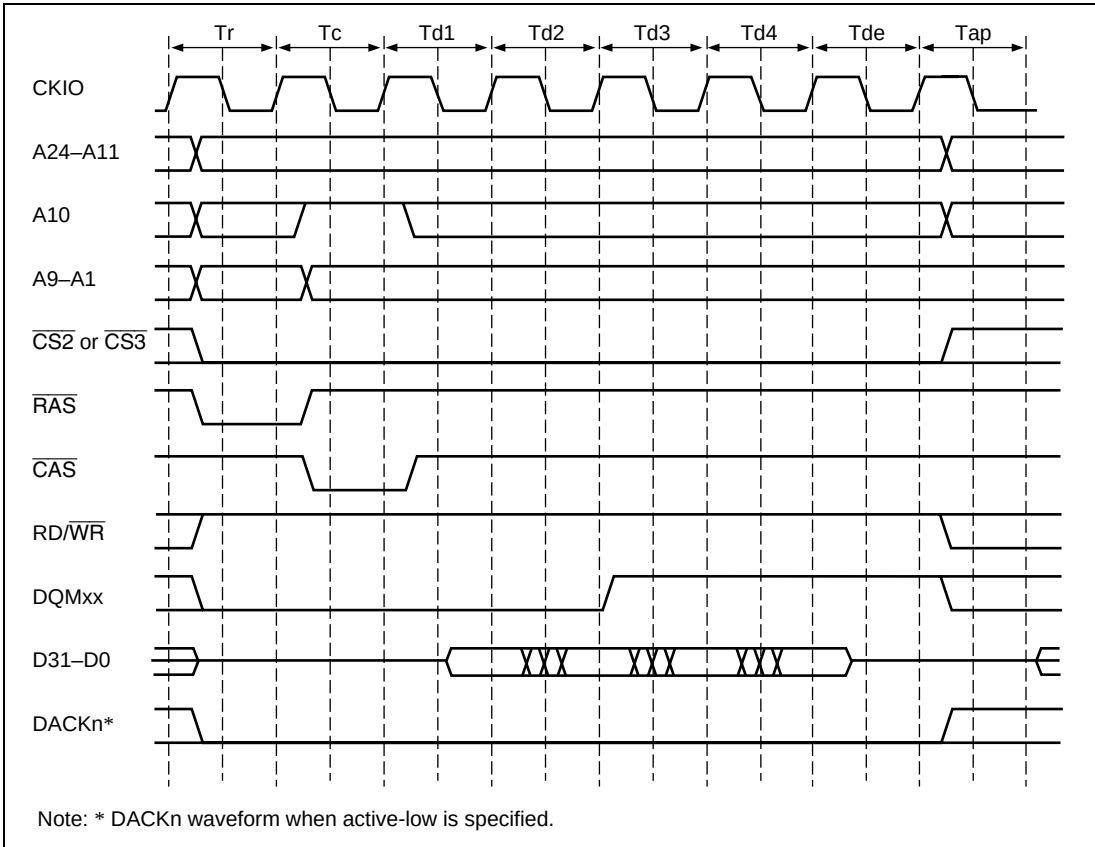
Figure 7.21 (a) Single Read Timing (Auto-Precharge) Except t_{E_{cyc}}:t_{P_{cyc}} 1:1
