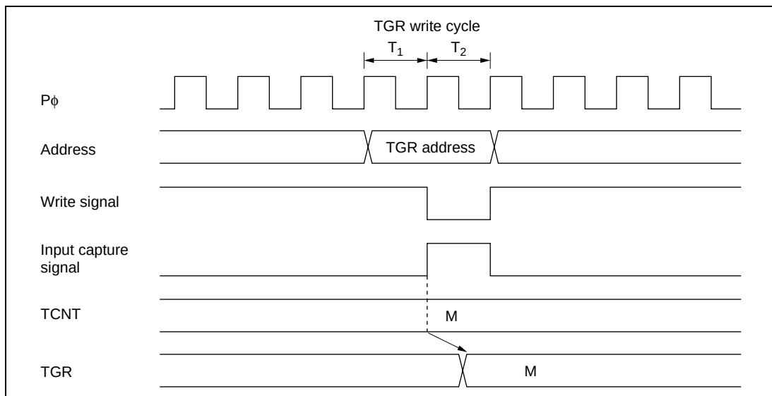
Figure 16.50 Contention between TGR Write and Input Capture
