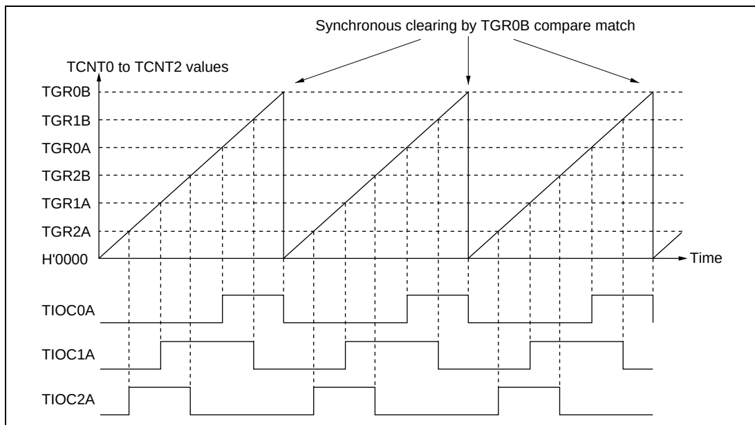
Figure 16.15 Example of Synchronous Operation
