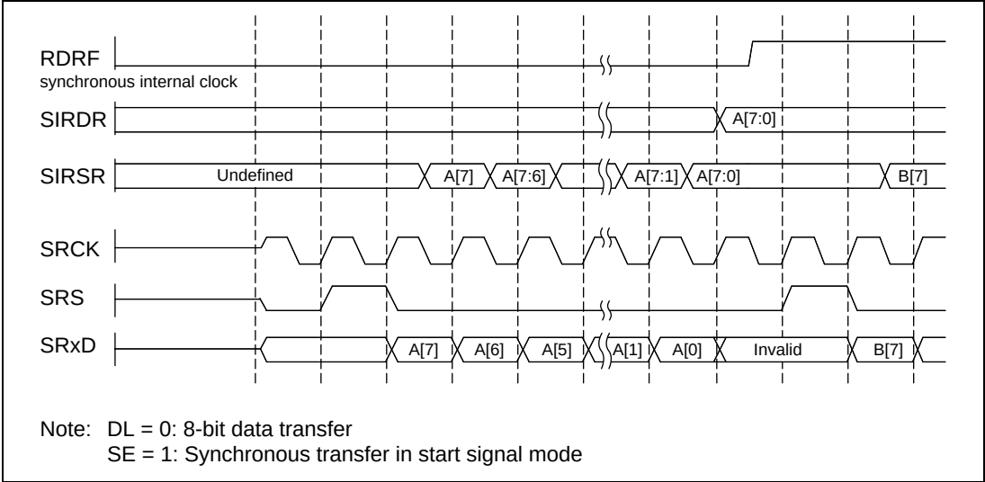
Figure 15.2 Reception: Interval Transfer Mode
