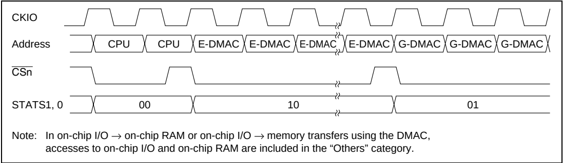
Figure 7.59 STATS Output Timing
