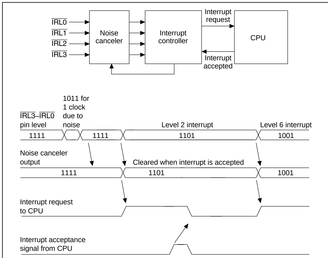
Figure 5.10 \overline{\text{IRL3}} to \overline{\text{IRL0}} Pin Sampling
