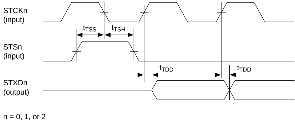
Figure 21.63 SIO Transmit Timing (TMn = 0 Mode)
