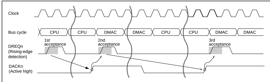
Figure 11.33 DREQn/DACKn Handshaking
