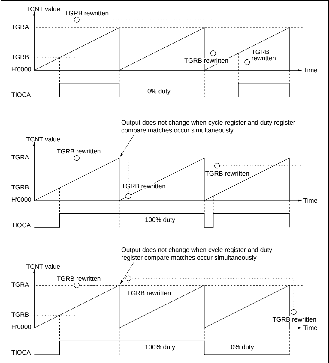
Figure 16.24 Example of PWM Mode Operation (3)
