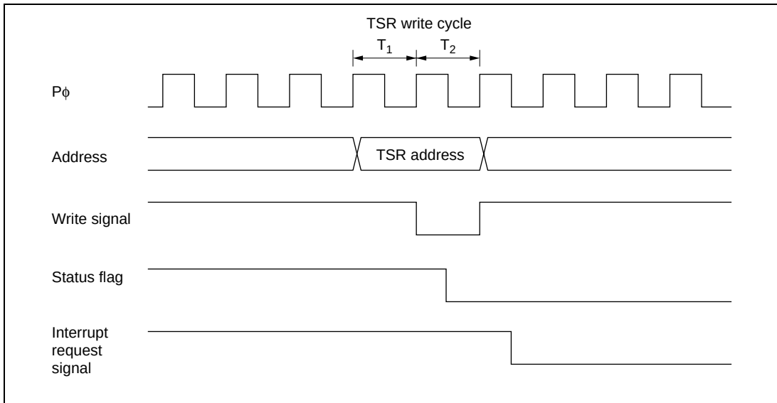
Figure 16.42 Timing for Status Flag Clearing by CPU
