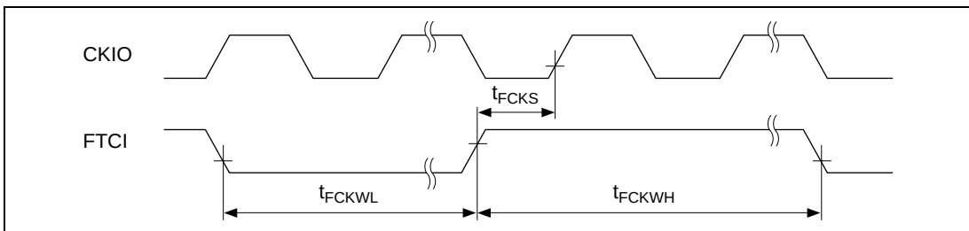
Figure 21.51 FRT Clock Input Timing ( t_{E_{cyc}}:t_{p_{cyc}} = 1:1 )
