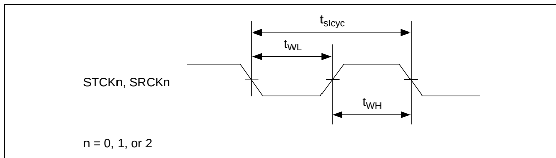
Figure 21.61 SIO Input Clock Timing
