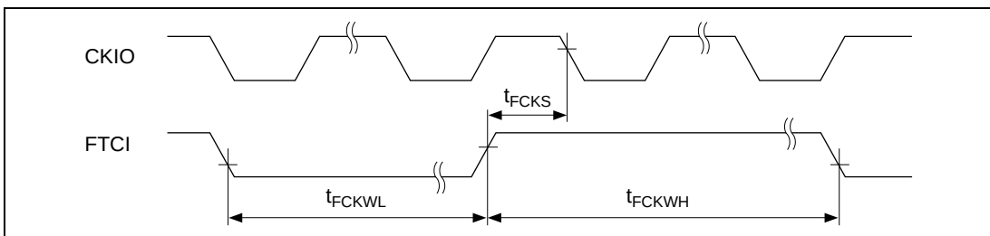
Figure 21.52 FRT Clock Input Timing (Except t_{E_{cyc}}:t_{p_{cyc}} 1:1)
