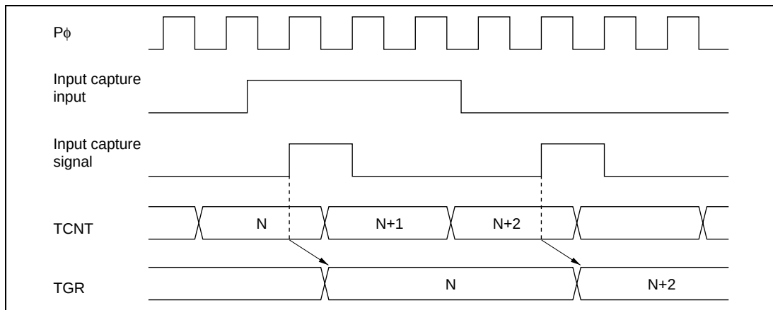
Figure 16.33 Input Capture Input Signal Timing
