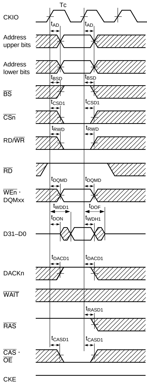
Figure 21.25 Synchronous DRAM Write Bus Cycle (Bank Active, Same Row Access, Except t_{E_{cyc}}:t_{P_{cyc}} 1:1)
