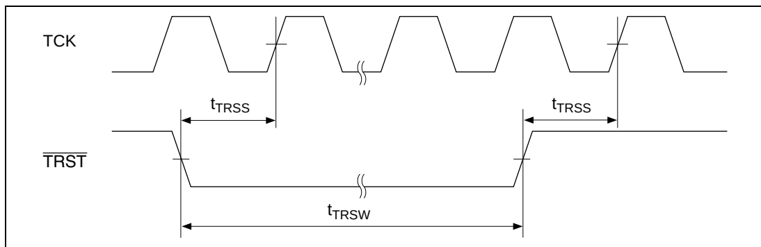
Figure 21.66 H-UDI \overline{\text{TRST}} Timing
