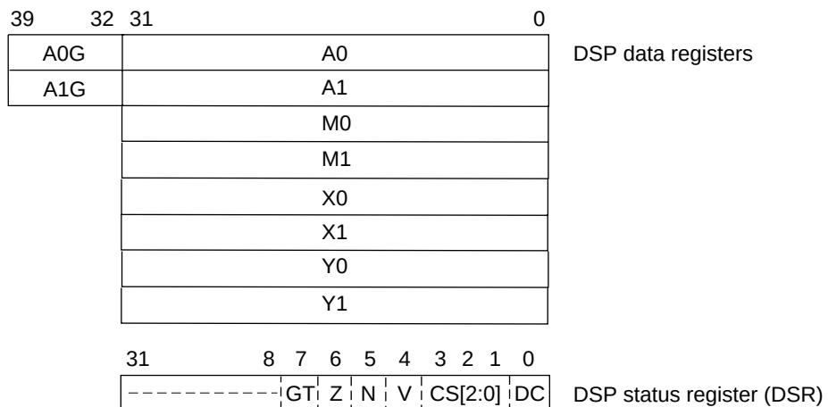
Figure 2.4 DSP Register Configuration
