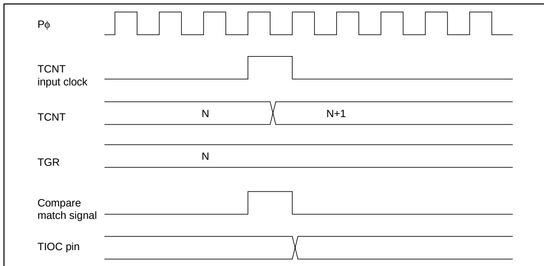
Figure 16.32 Output Compare Output Timing
