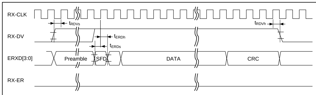
Figure 21.72 MII Receive Timing (Normal Operation)
