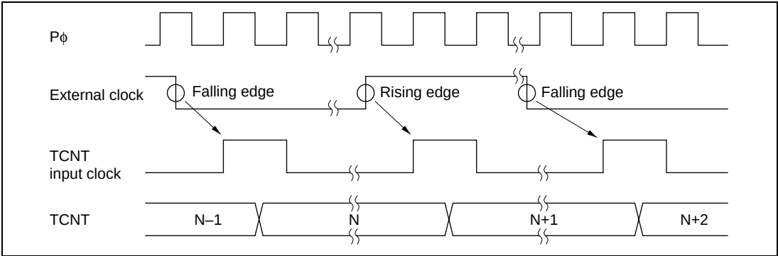
Figure 16.31 Count Timing in External Clock Operation
