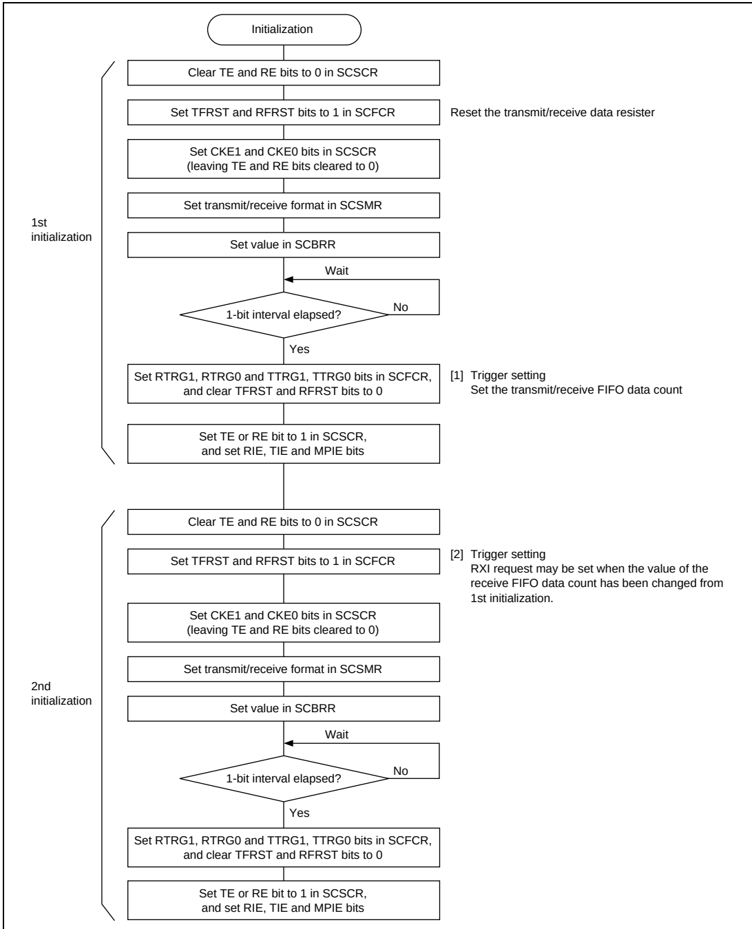
Figure 14.27 Example of SCIF Initialization Flowchart
