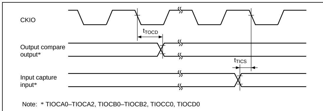
Figure 21.57 TPU Input/Output Timing (Except t_{E_{cyc}}:t_{P_{cyc}} 1:1 )
