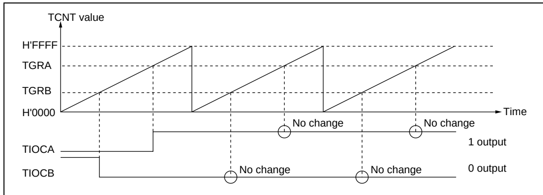
Figure 16.10 Example of 0 Output/1 Output Operation
