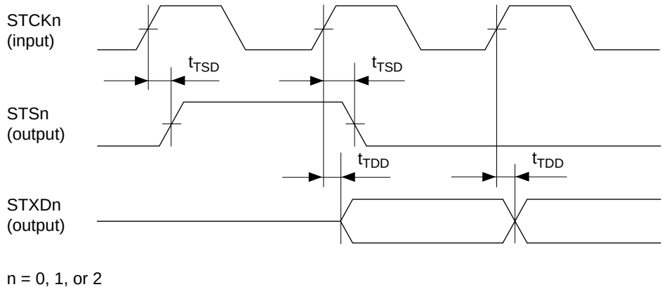
Figure 21.64 SIO Transmit Timing (TMn = 1 Mode)
