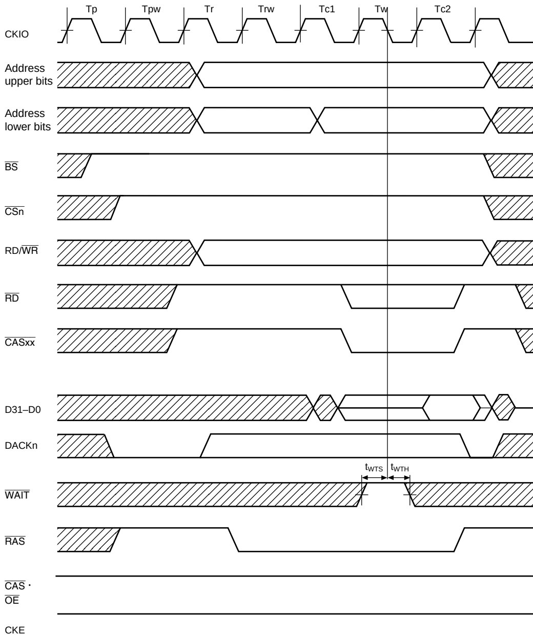
Figure 21.36 DRAM Bus Cycle (TRP = 2 Cycles, RCD = 2 Cycles, 1 Wait)
