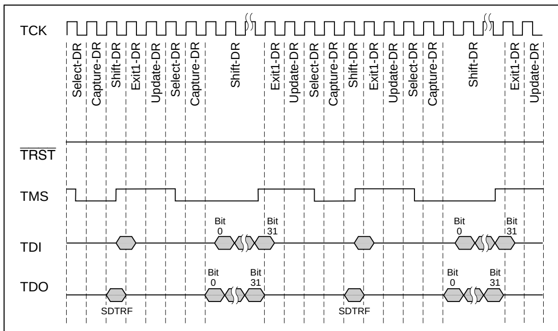
Figure 17.5 Data Input/Output Timing Chart (3)
