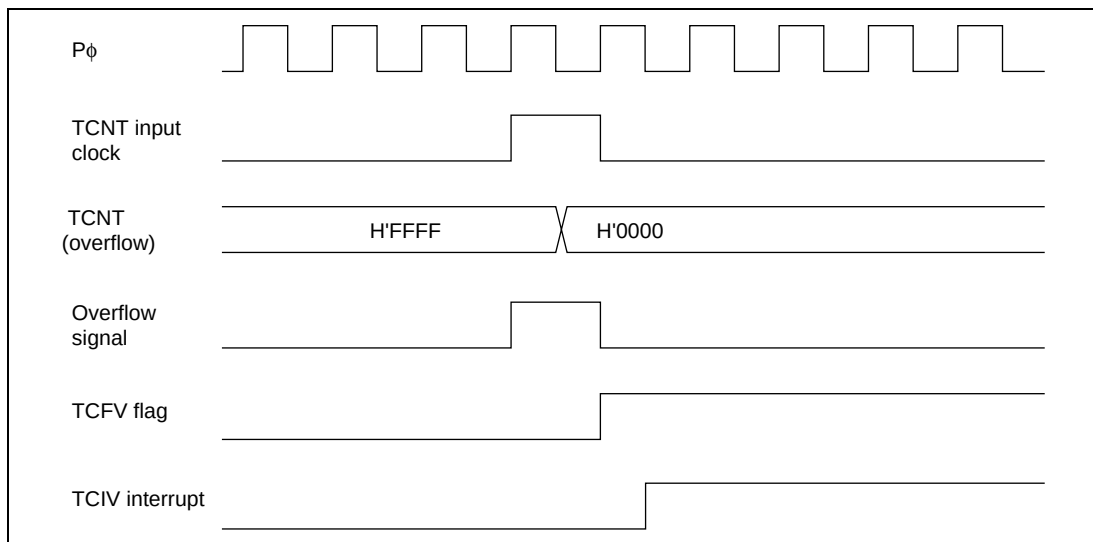
Figure 16.40 TCIV Interrupt Setting Timing
