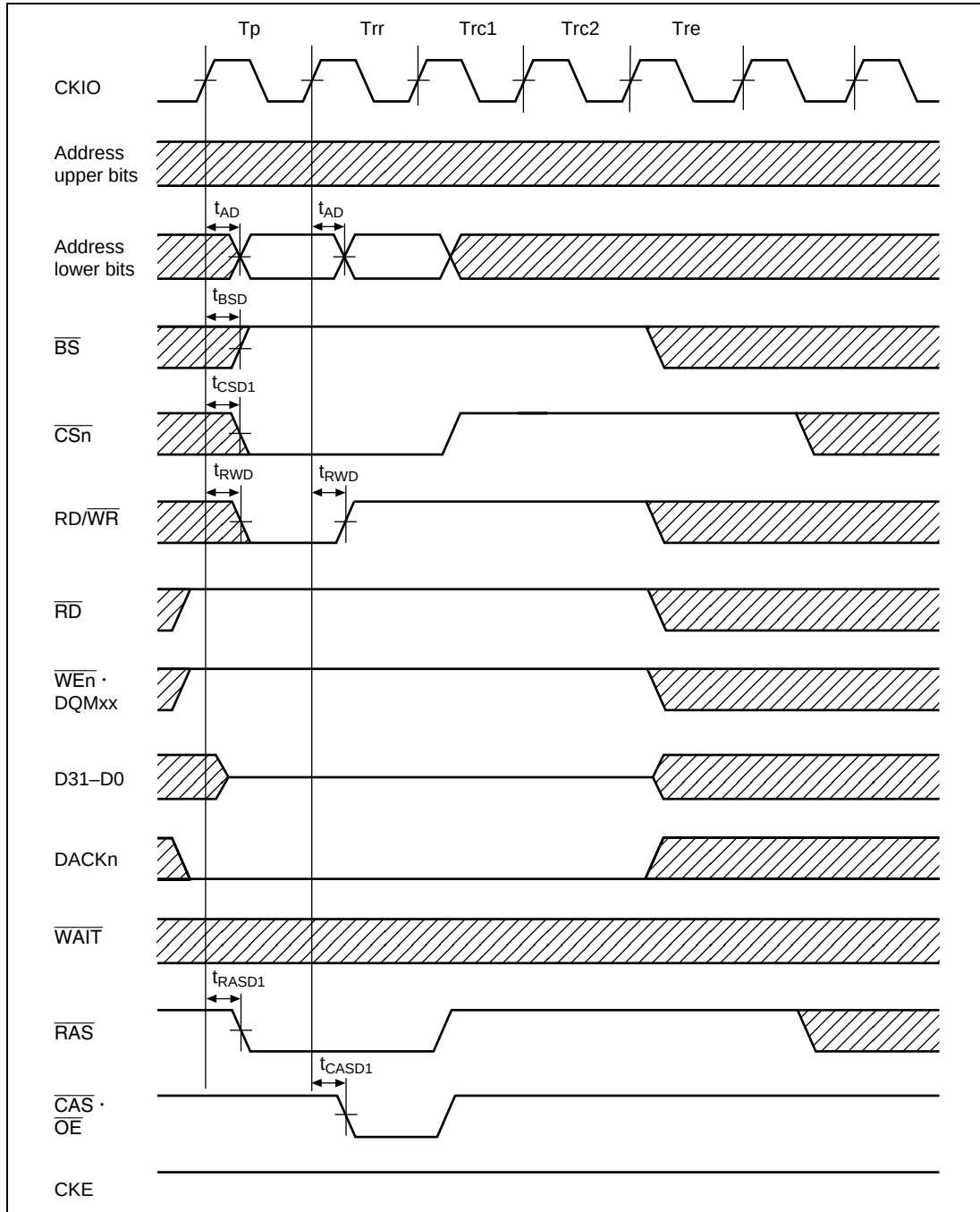
Figure 21.32 Synchronous DRAM Auto-Refresh Cycle (Shown from Precharge Cycle, TRP = 1 Cycle, TRAS = 4 Cycles)
