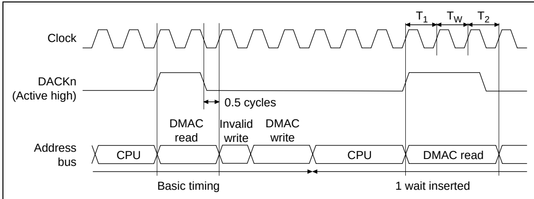
Figure 11.14 DACKn Output in Ordinary Space Accesses (AM = 0)
