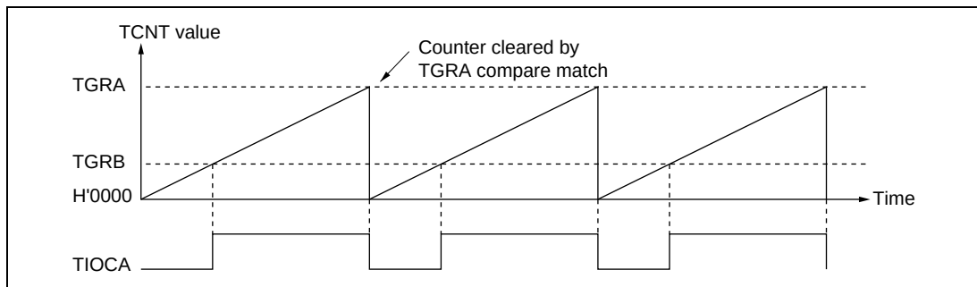
Figure 16.22 Example of PWM Mode Operation (1)
