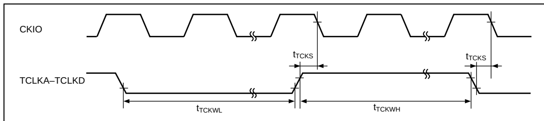
Figure 21.58 TPU Clock Input Timing
