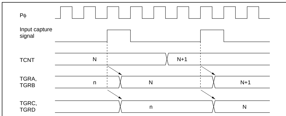
Figure 16.37 Buffer Operation Timing (Input Capture)
