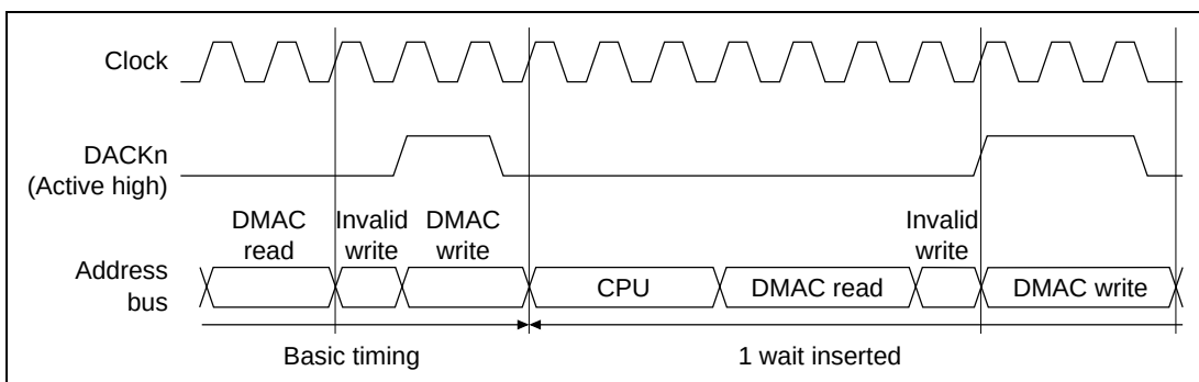
Figure 11.15 DACKn Output in Ordinary Space Accesses (AM = 1)
