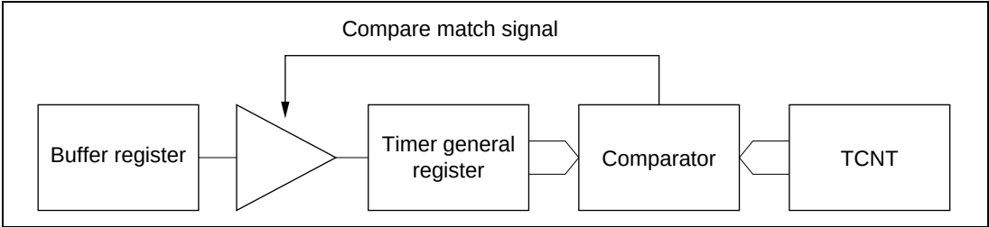
Figure 16.16 Compare Match Buffer Operation
