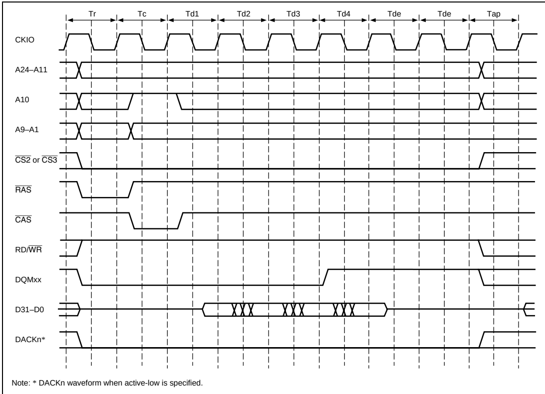
Figure 7.21 (b) Single Read Timing (Auto-Precharge) I\phi:E\phi = 1:1
