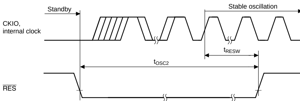
Figure 21.5 Power-On Oscillation Stabilization Time at Power-On
