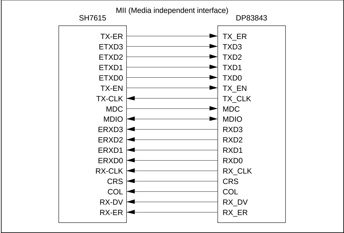
Figure 9.8 Example of Connection to DP83843
