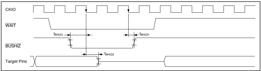
Figure 21.80 BUSHiZ Bus Timing
