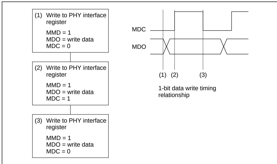
Figure 9.6 (a) 1-Bit Data Write Flowchart
