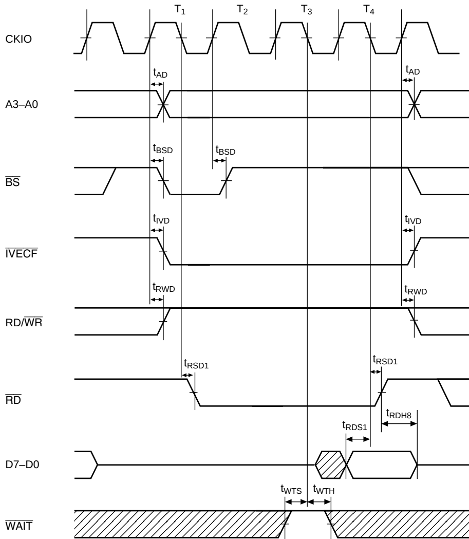
Figure 21.44 Interrupt Vector Fetch Cycle (No Wait, Iφ:Eφ = 1:1)
