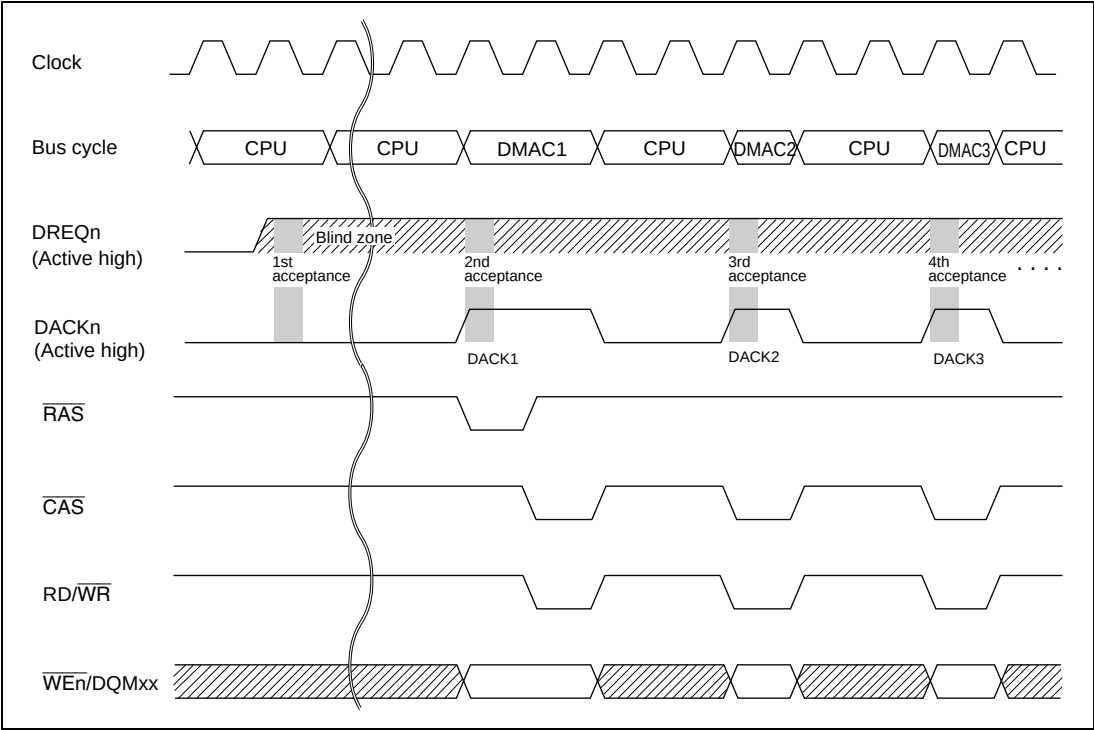
Figure 11.28 (a) Synchronous DRAM One-Cycle Write Timing
