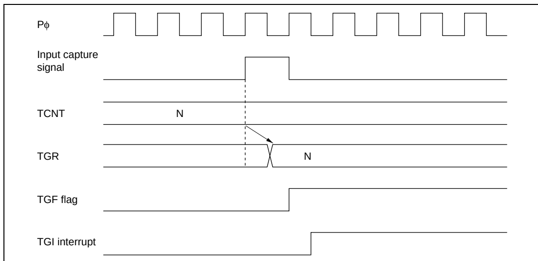
Figure 16.39 TGI Interrupt Timing (Input Capture)
