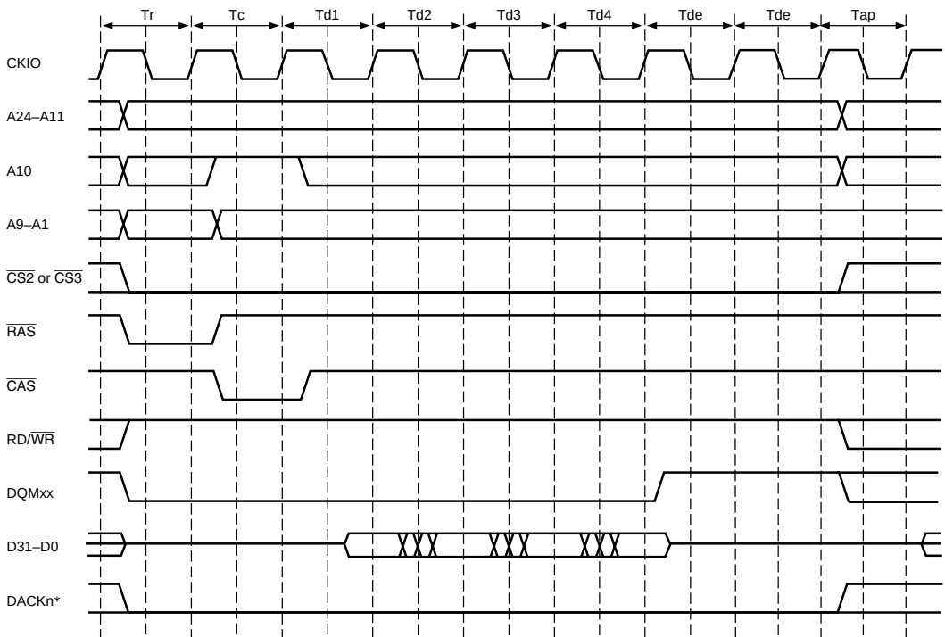
Figure 7.19 (b) Basic Burst Read Timing (Auto-Precharge) I\phi:E\phi = 1:1
