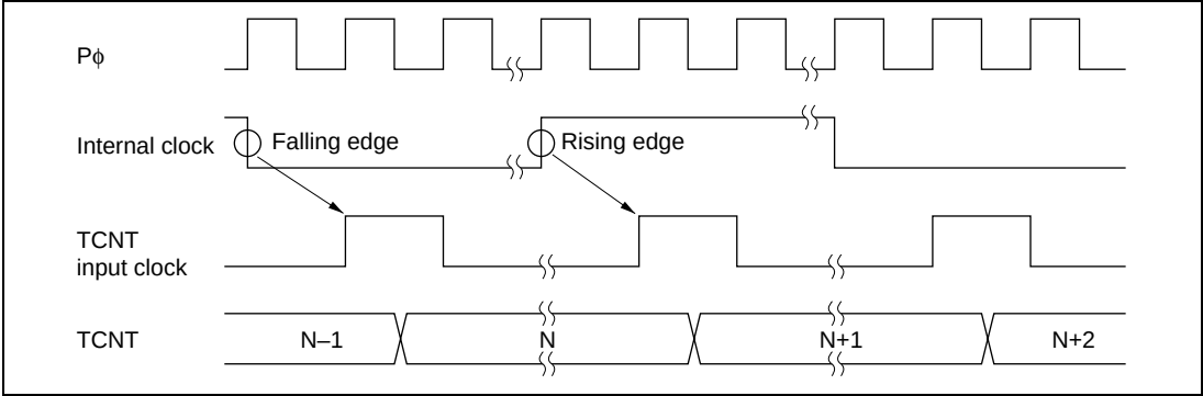
Figure 16.30 Count Timing in Internal Clock Operation
