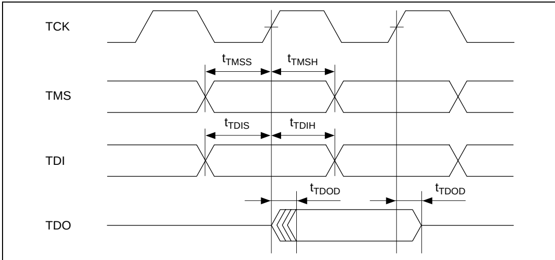
Figure 21.67 H-UDI Input/Output Timing
