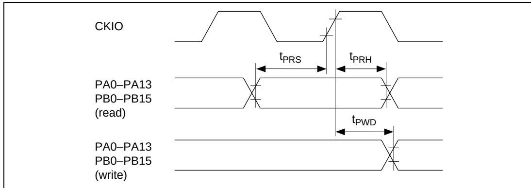
Figure 21.68 I/O Port Input/Output Timing ( t_{E_{cyc}}:t_{P_{cyc}} = 1:1 )
