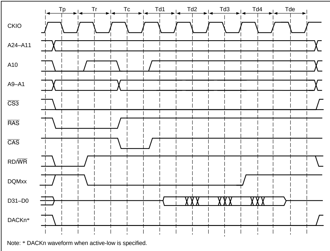
Figure 7.26 (a) Burst Read Timing (Bank Active, Different Row Addresses) Except t_{E_{cyc}}:t_{P_{cyc}} 1:1
