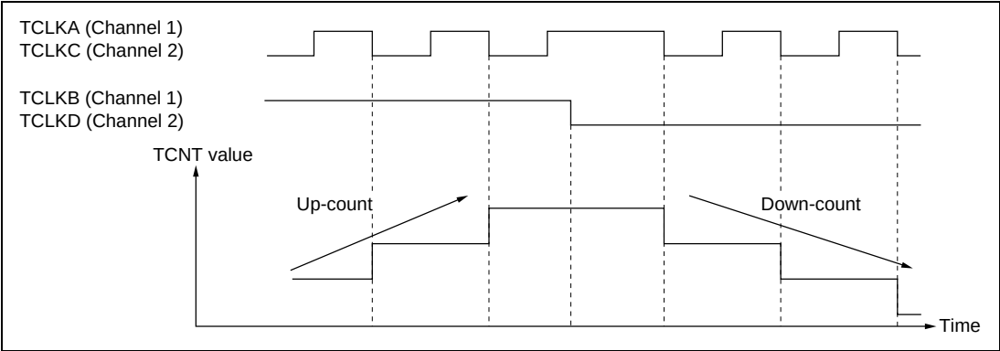
Figure 16.27 Example of Phase Counting Mode 2 Operation
