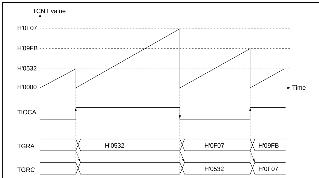
Figure 16.20 Example of Buffer Operation (2)
