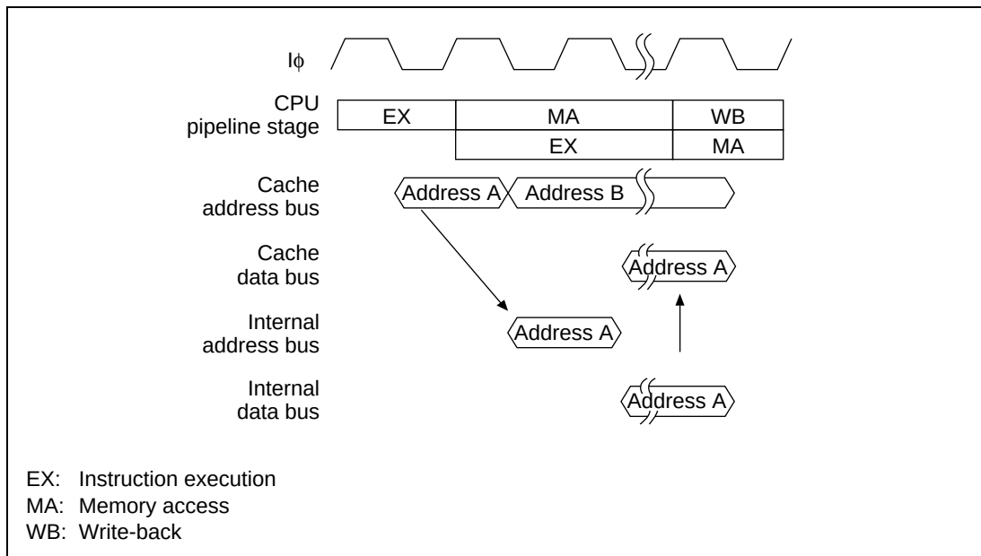
Figure 8.9 Reading Cache-Through Areas
