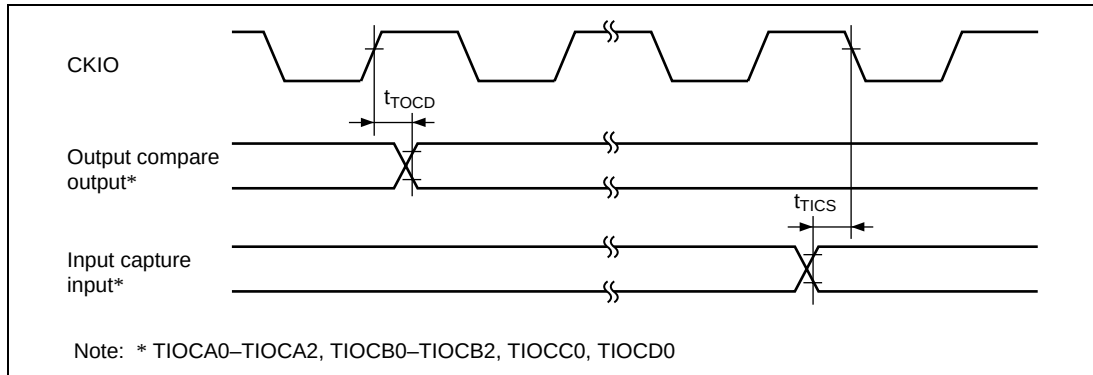
Figure 21.56 TPU Input/Output Timing ( t_{E_{cyc}}:t_{P_{cyc}} = 1:1 )
