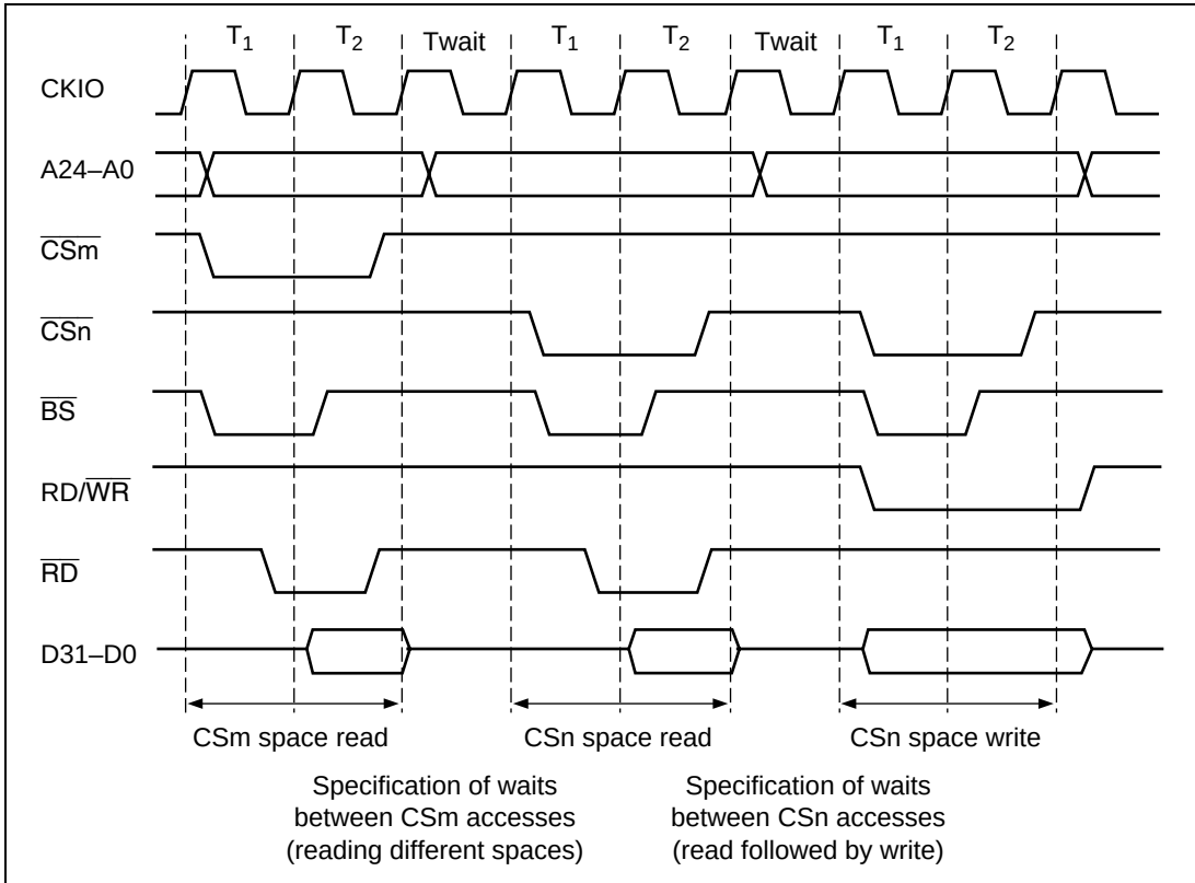
Figure 7.56 Idles between Cycles
