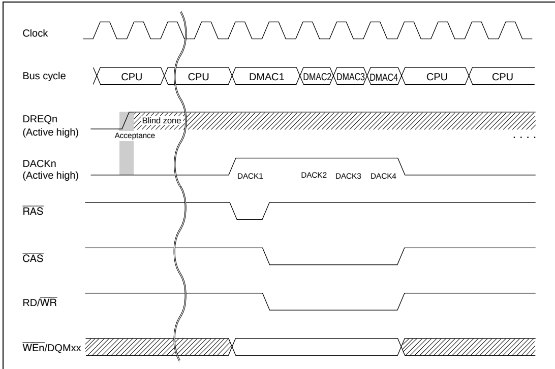
Figure 11.28 (b) Synchronous DRAM One-Cycle Write Timing
