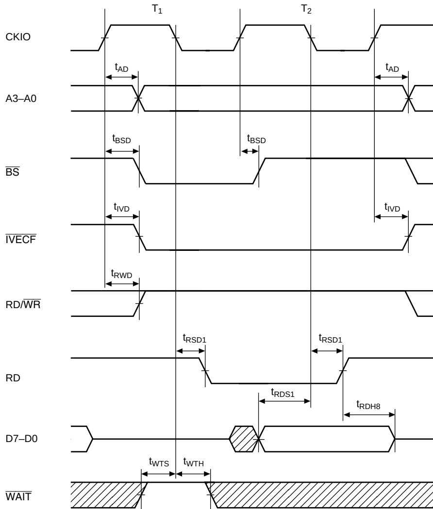
Figure 21.45 Interrupt Vector Fetch Cycle (No Wait, Except t_{E\text{cyc}}:t_{P\text{cyc}} 1:1)
