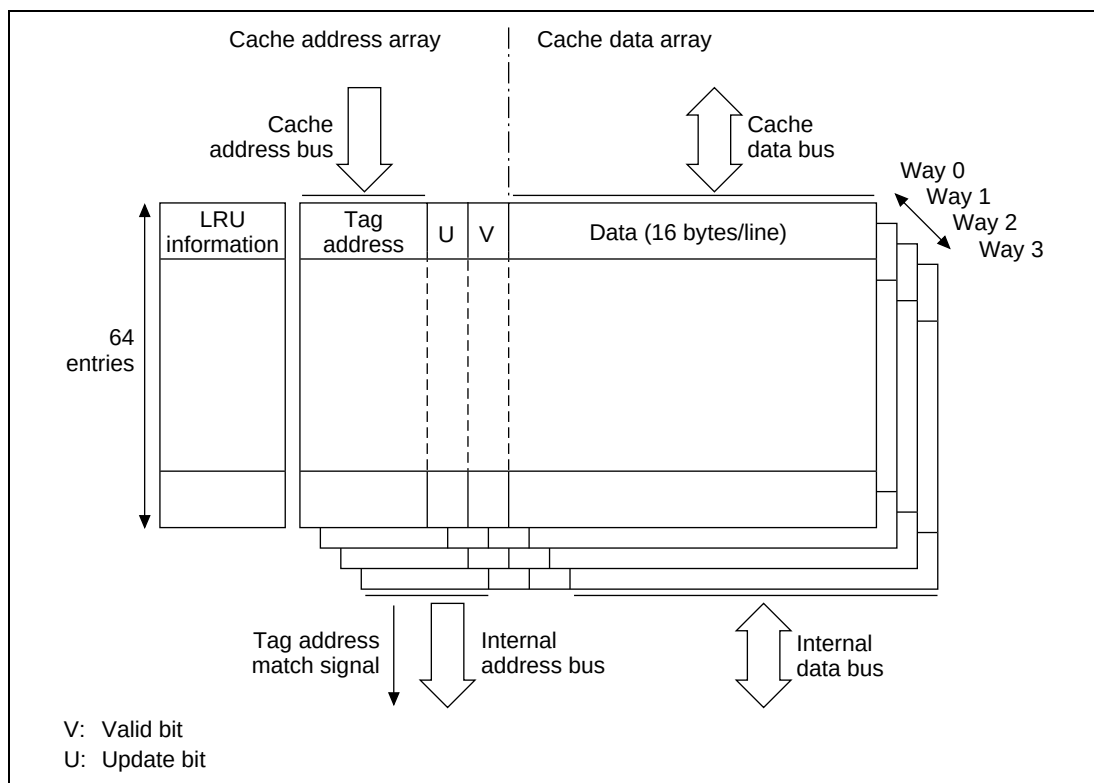
Figure 8.1 Cache Configuration
