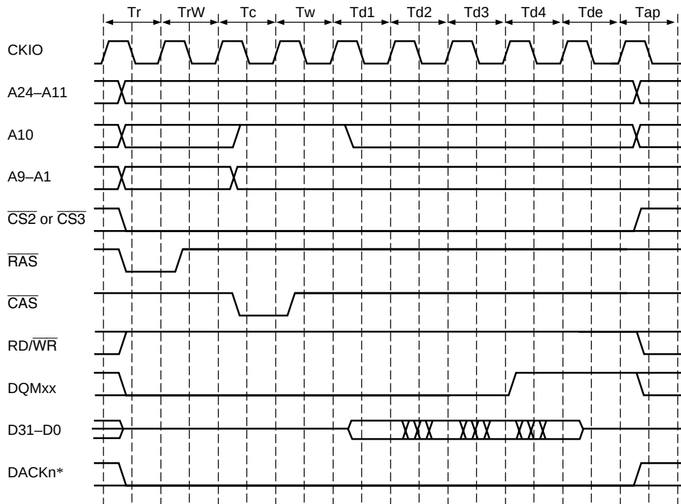
Figure 7.20 (a) Burst Read Wait Specification Timing (Auto-Precharge) Except t_{Eyc} \cdot t_{p_{yc}} 1:1
