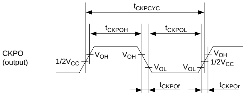
Figure 21.4 CKPO Clock Output Timing
