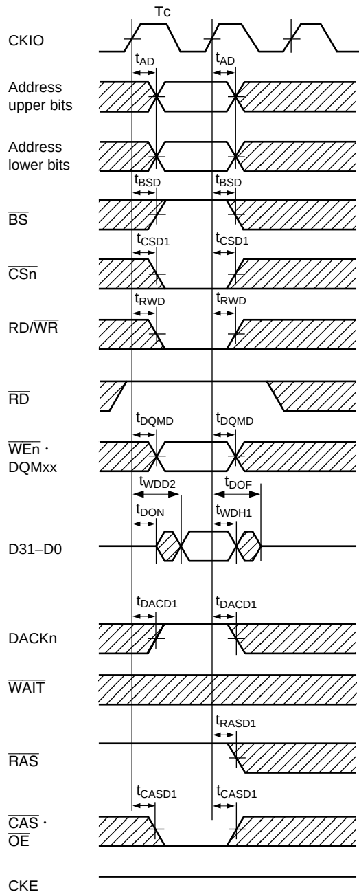
Figure 21.26 Synchronous DRAM Write Cycle (Bank Active, Same Row Access, I φ :E φ = 1:1)
