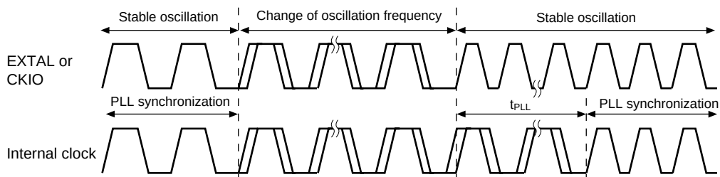
Figure 21.8 PLL Synchronization Stabilization Time
