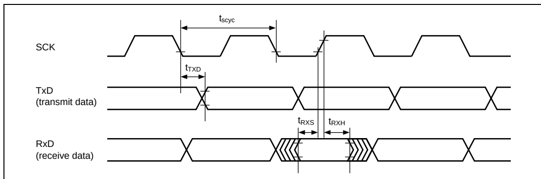
Figure 21.54 SCI Input/Output Timing (Synchronous Mode)
