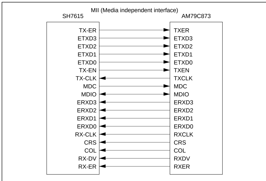
Figure 9.7 Example of Connection to AM79C873
