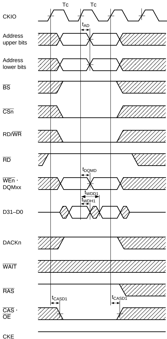
Figure 21.27 Synchronous DRAM Continuous Write Cycle (Bank Active, Same Row Access, Except t_{Eccyc}::t_{Pcyc} 1:1)
