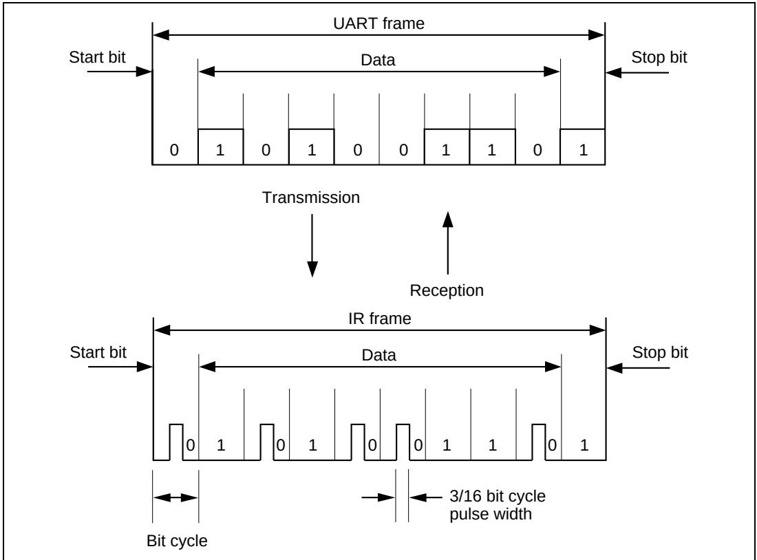
Figure 14.24 IrDA Mode Transmit/Receive Operations
