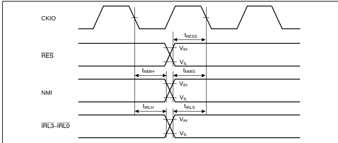
Figure 21.10 Interrupt Signal Input Timing
