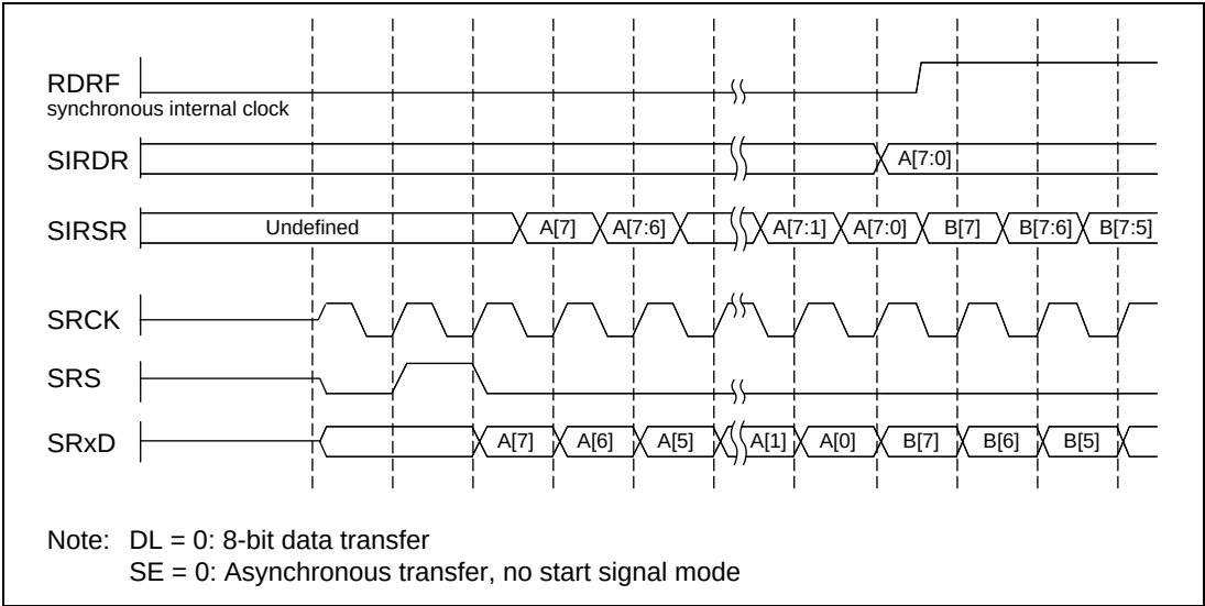
Figure 15.3 Reception: Continuous Transfer Mode
