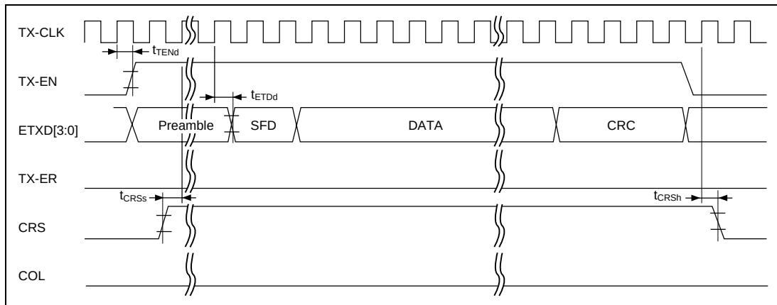
Figure 21.70 MII Transmit Timing (Normal Operation)
