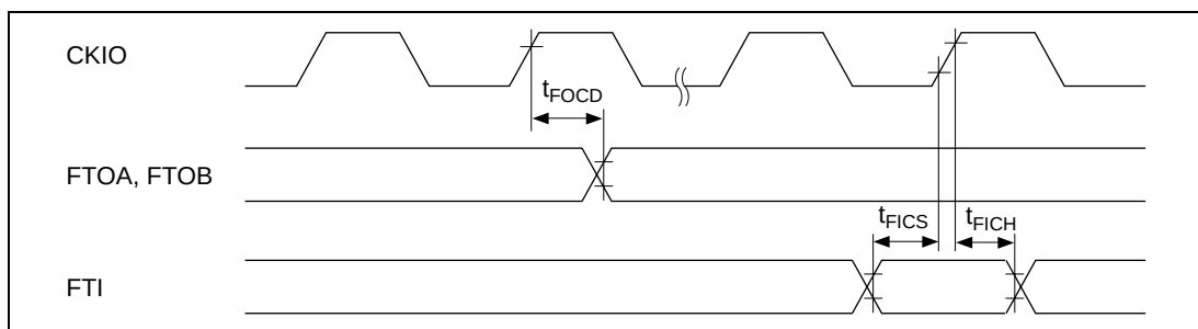
Figure 21.49 FRT Input/Output Timing ( t_{E_{cyc}}:t_{P_{cyc}} = 1:1 )
