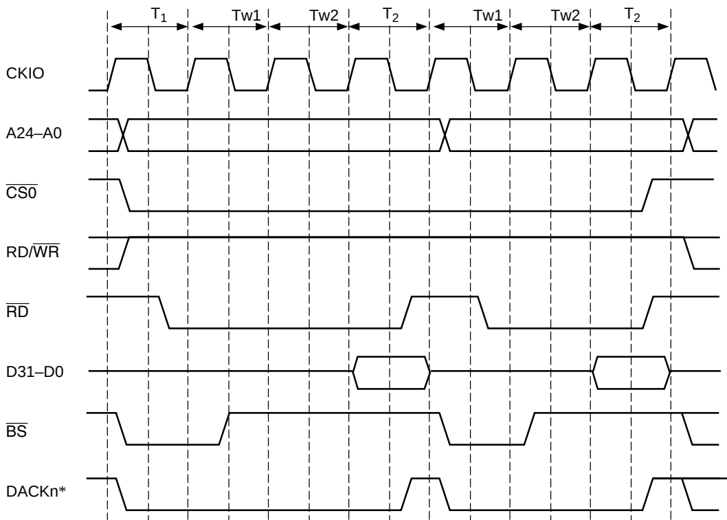
Figure 7.54 Burst ROM Nibble Access (2 Wait States)
