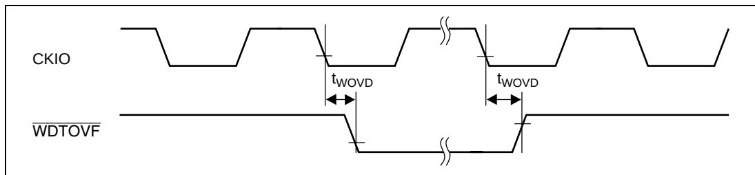
Figure 21.60 Watchdog Timer Output Timing (Except t_{E_{cyc}}:t_{P_{cyc}} 1:1 )
