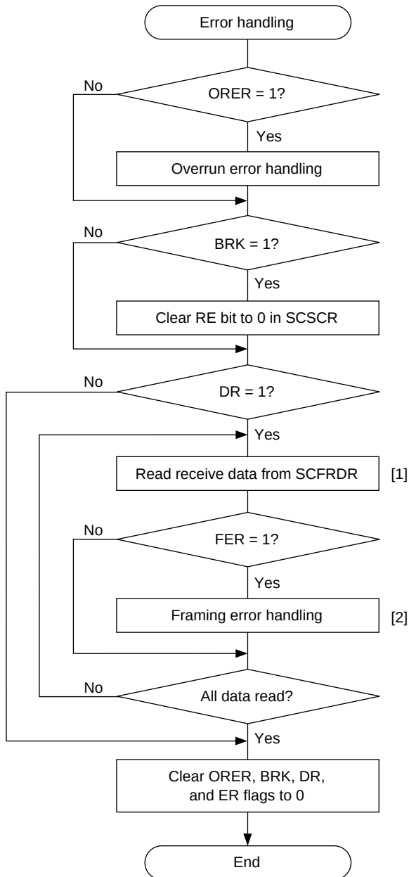
Figure 14.14 Sample Multiprocessor Serial Reception Flowchart (2)
