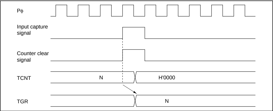
Figure 16.35 Counter Clear Timing (Input Capture)
