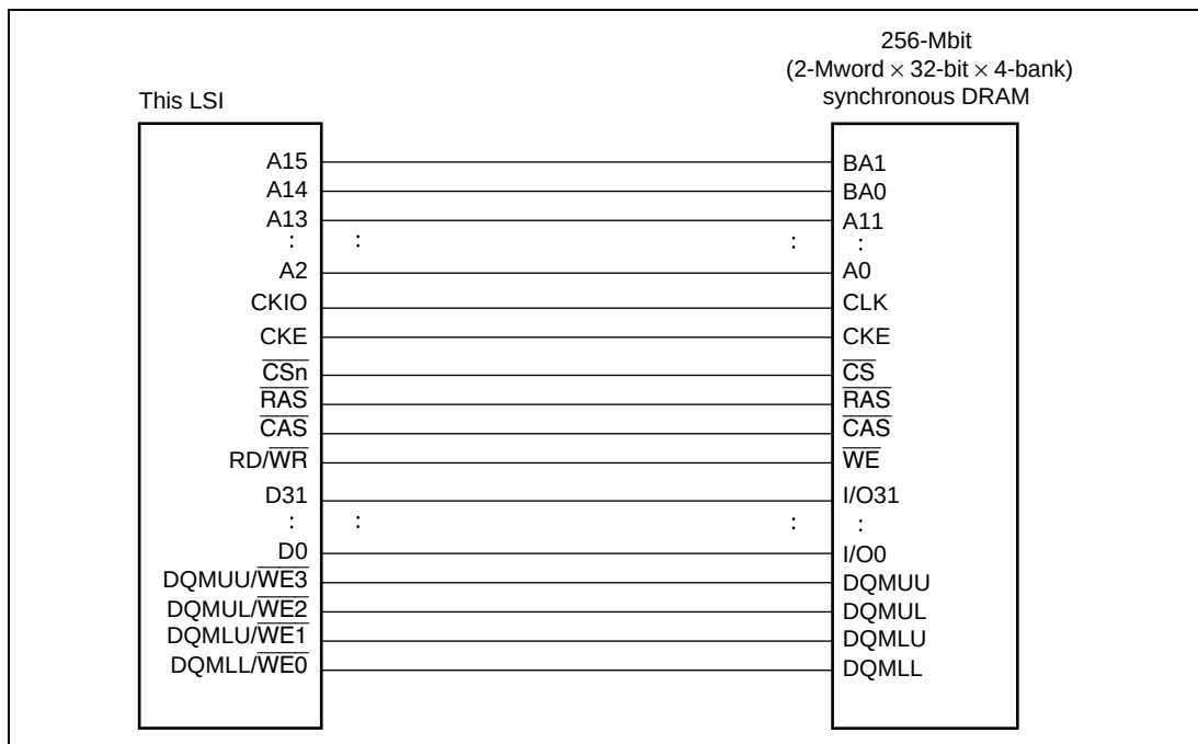
Figure 7.37 256-Mbit Synchronous DRAM (8 Mwords × 32 Bits) Connection Example
