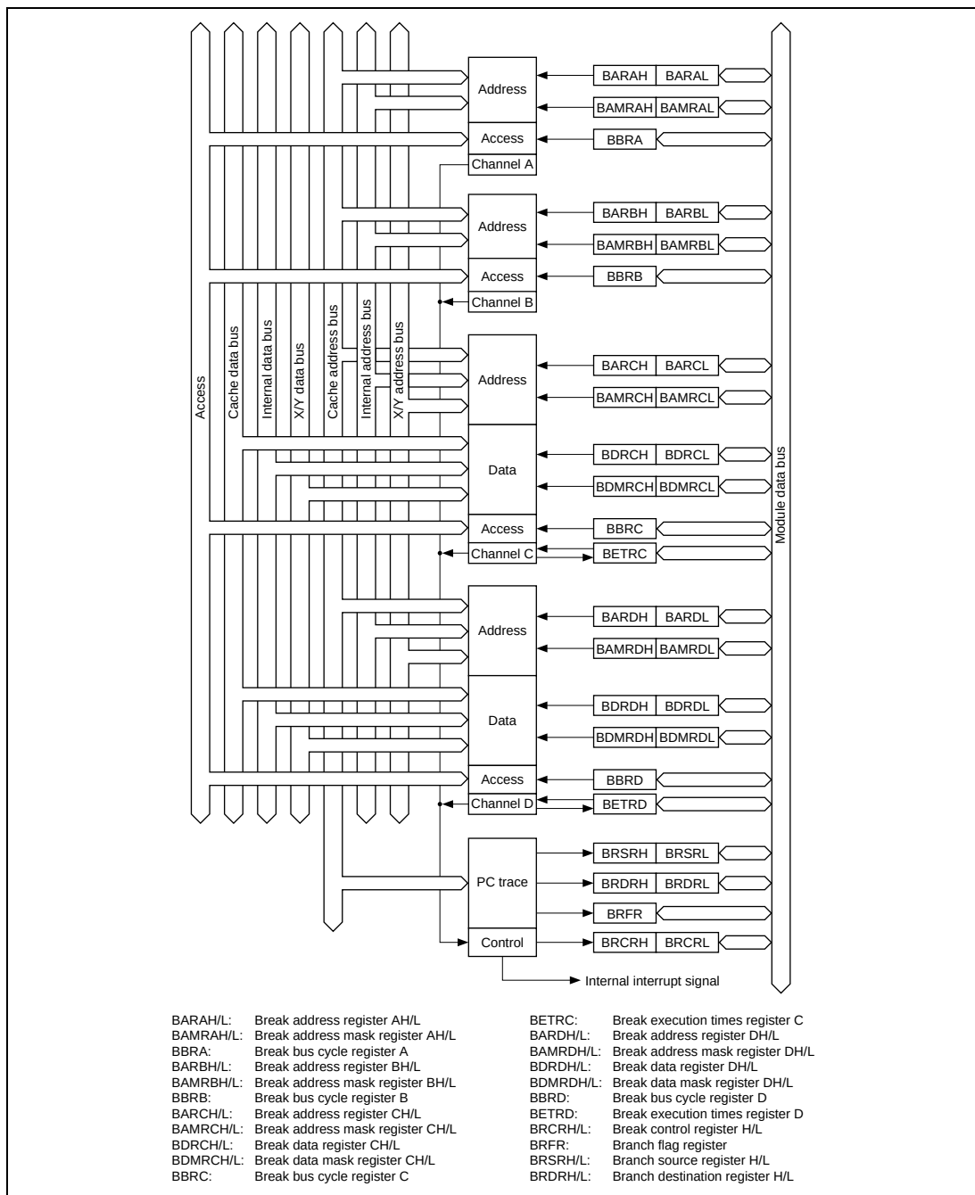
Figure 6.1 Block Diagram of User Break Controller
