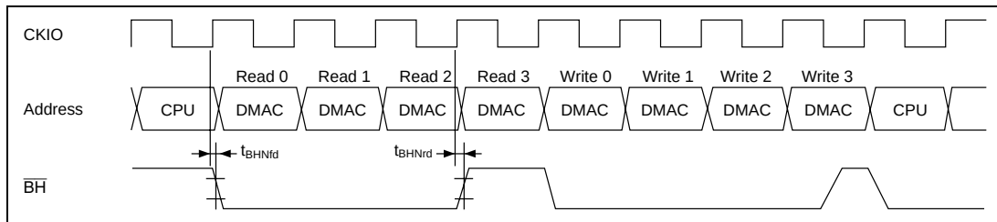
Figure 21.79 \overline{\text{BH}} Output Timing
