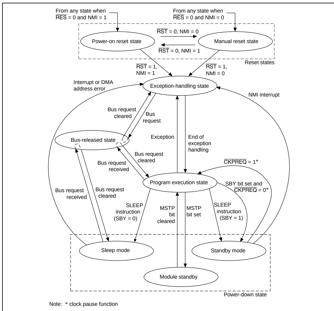
Figure 1.4 Processing State Transitions
