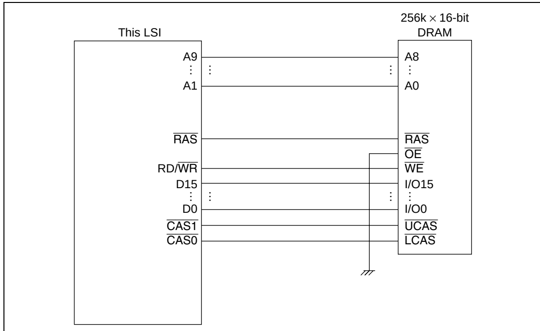
Figure 7.39 Example of DRAM Connection (16-Bit Data Width)
