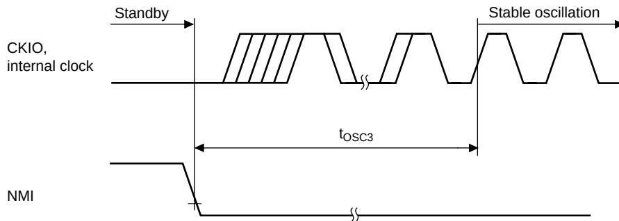
Figure 21.7 Oscillation Stabilization Time after Standby Recovery (Recovery by NMI)
