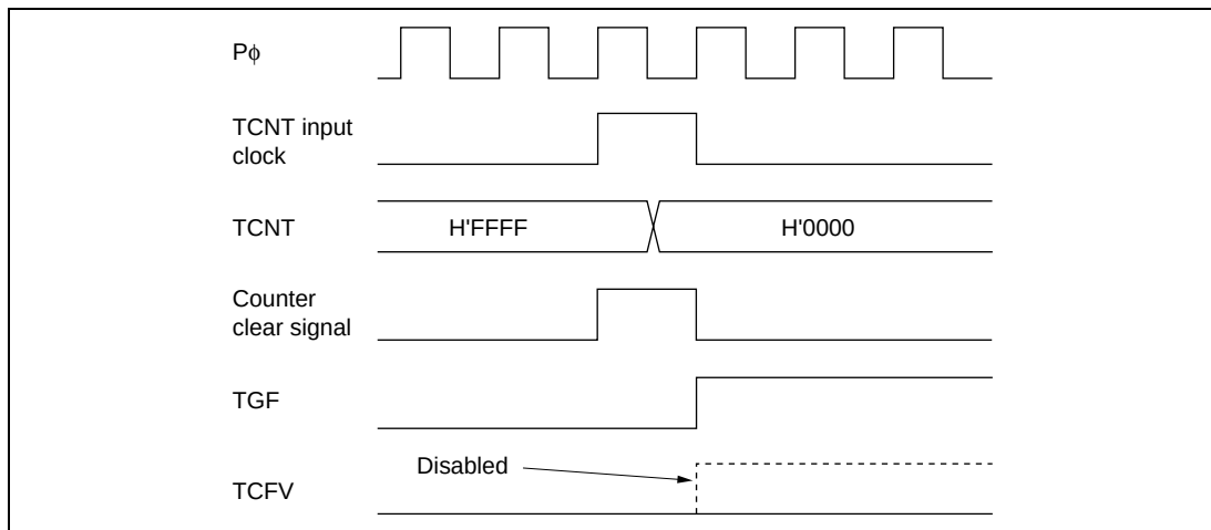
Figure 16.52 Contention between Overflow and Counter Clearing
