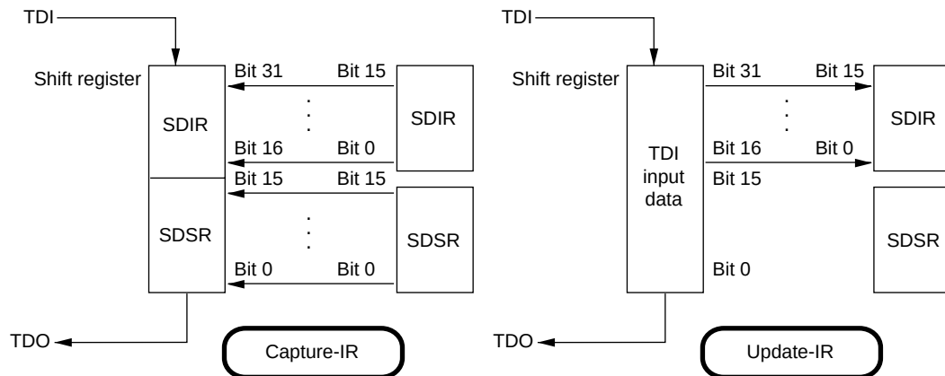
Figure 17.6 Serial Data Input/Output (1)
