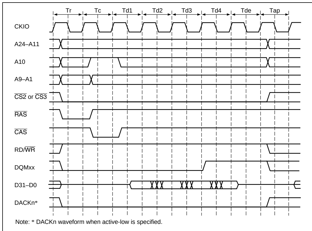
Figure 7.19 (a) Basic Burst Read Timing (Auto-Precharge) Except t_{E_{cyc}}:t_{P_{cyc}} 1:1
