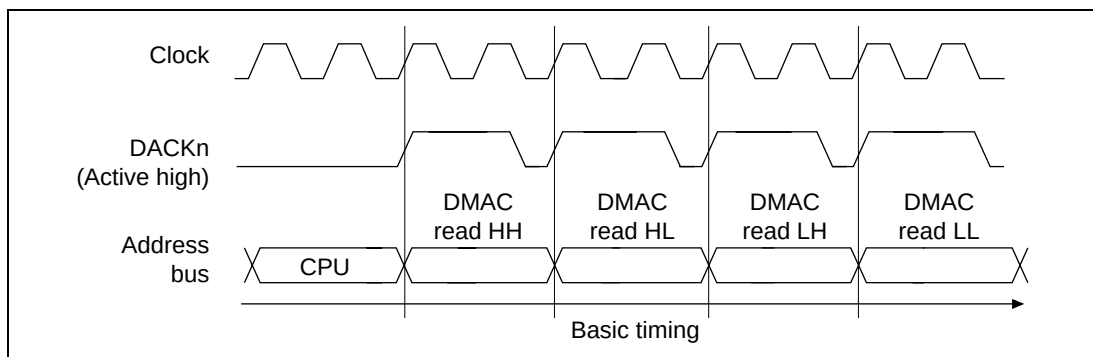
Figure 11.17 DACKn Output in Ordinary Space Accesses (AM = 0, Longword Access to 8-Bit External Device)
