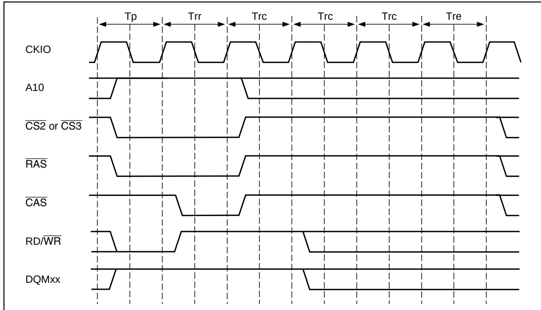
Figure 7.30 Auto-Refresh Timing
