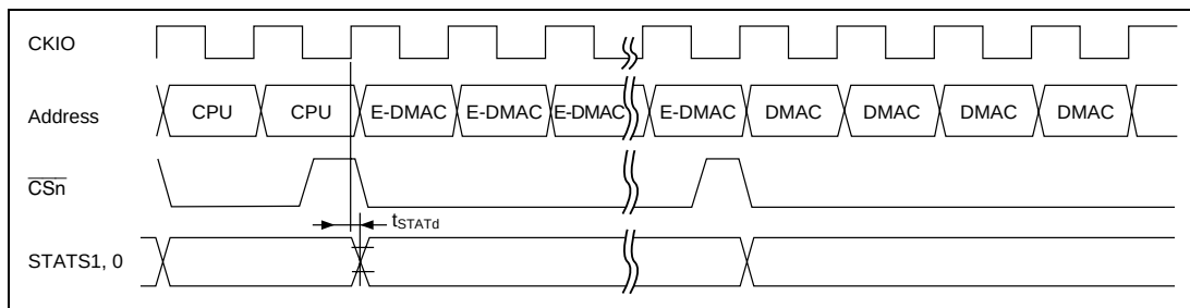
Figure 21.78 STATS Output Timing
