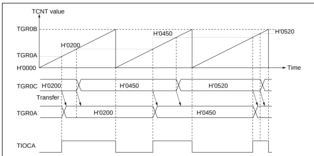
Figure 16.19 Example of Buffer Operation (1)
