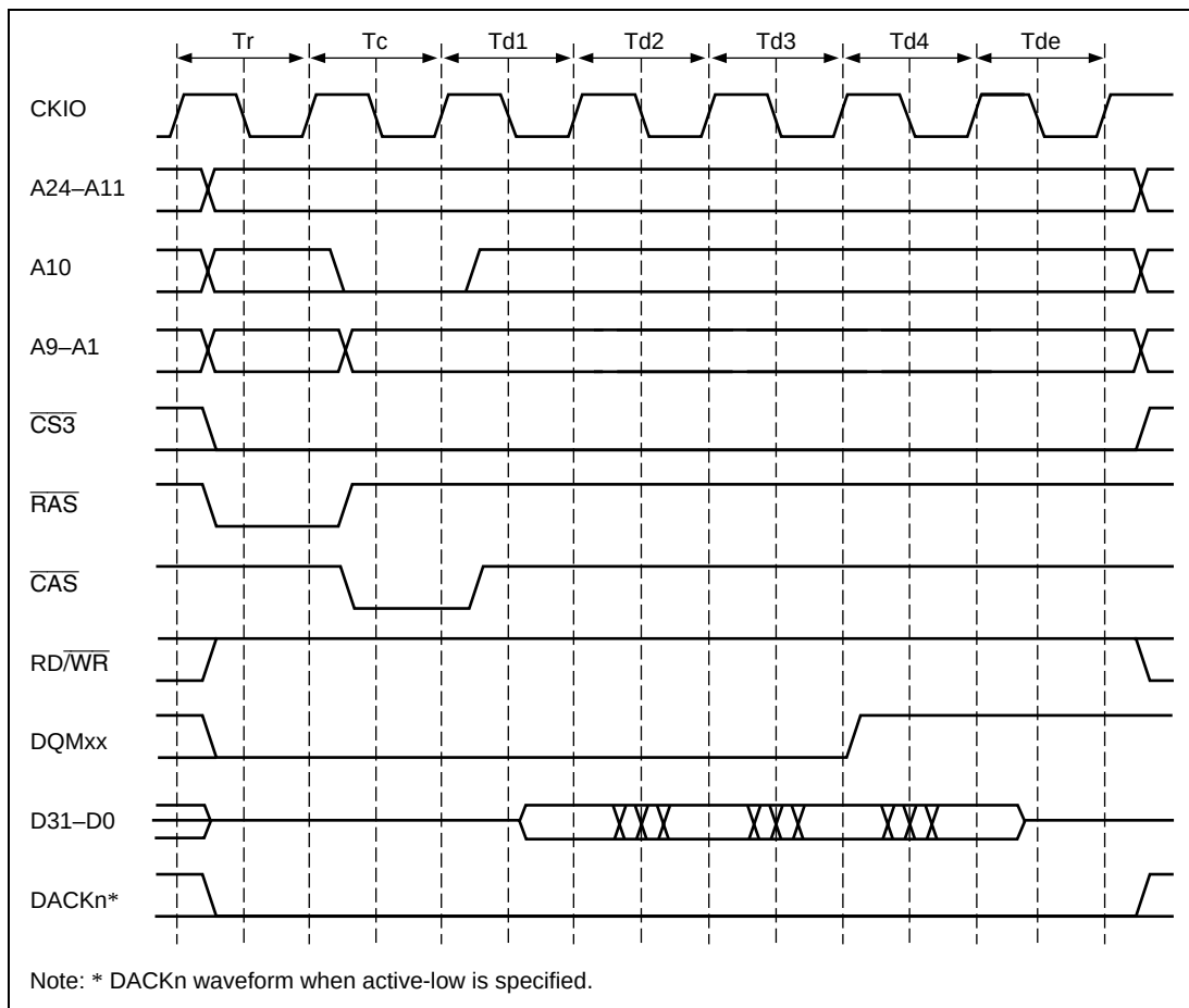
Figure 7.24 (a) Burst Read Timing (No Precharge) Except t_{E_{cyc}}:t_{P_{cyc}} 1:1
