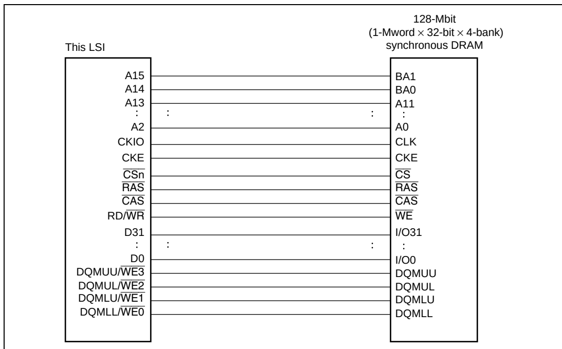
Figure 7.35 128-Mbit Synchronous DRAM (4 Mwords \times 32 Bits) Connection Example
