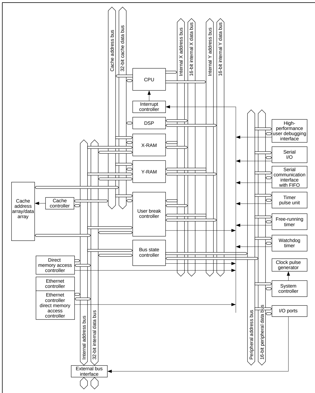
Figure 1.1 Block Diagram of SH7615
