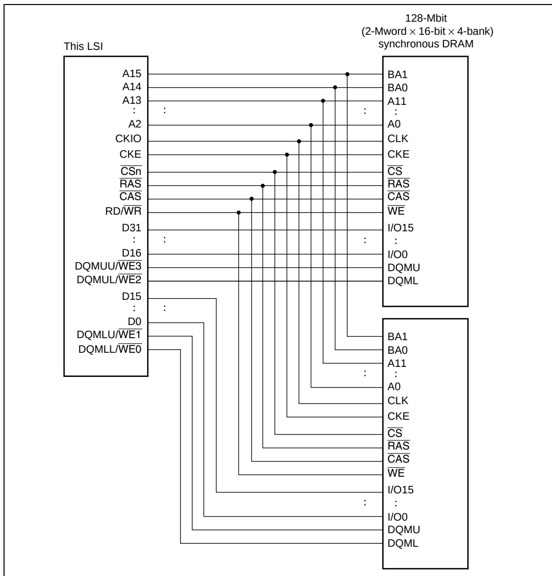
Figure 7.36 128-Mbit Synchronous DRAM (8 Mwords × 16 Bits) Connection Example
