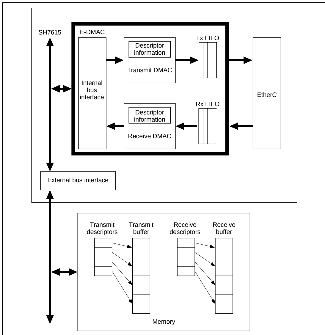
Figure 10.1 Configuration of E-DMAC, and Descriptors and Buffers
