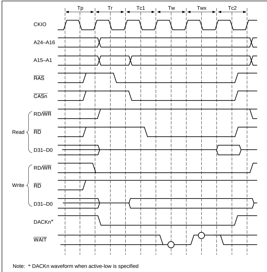
Figure 7.42 External Wait State Timing
