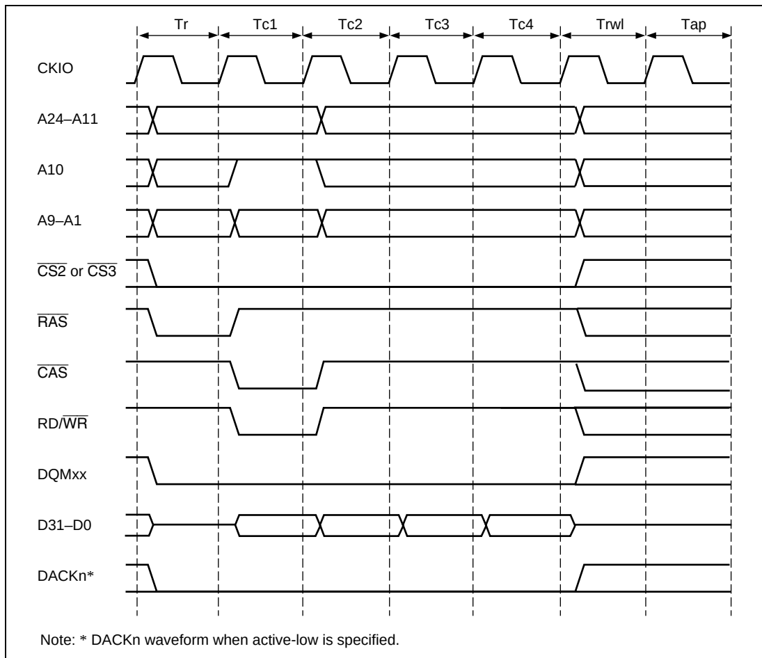
Figure 7.23 (a) Basic Burst Write Timing (Auto-Precharge) Except t_{E_{cyc}}:t_{P_{cyc}} 1:1
