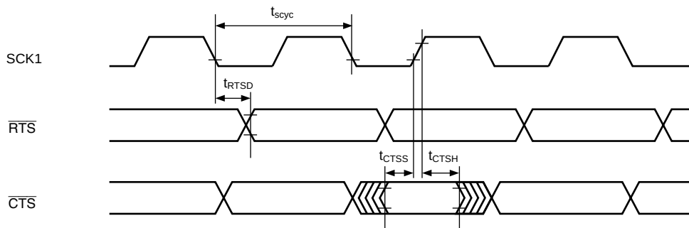
Figure 21.55 \overline{\text{RTS}} and \overline{\text{CTS}} Input/Output Timing
