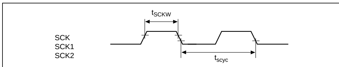
Figure 21.53 Input Clock Input/Output Timing
