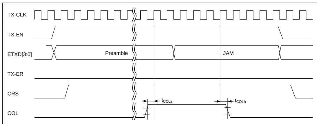
Figure 21.71 MII Transmit Timing (Case of Conflict)
