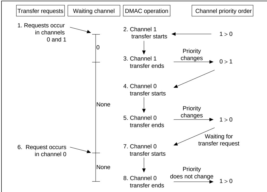
Figure 11.5 Channel Priority in Round-Robin Mode
