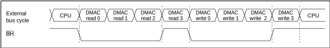
Figure 11.43 Summary of \overline{\text{BH}} Output Timing
