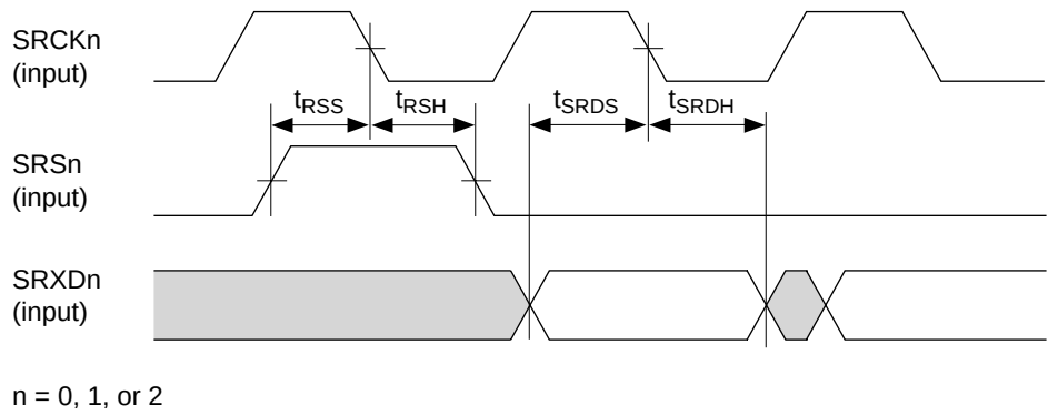
Figure 21.62 SIO Receive Timing
