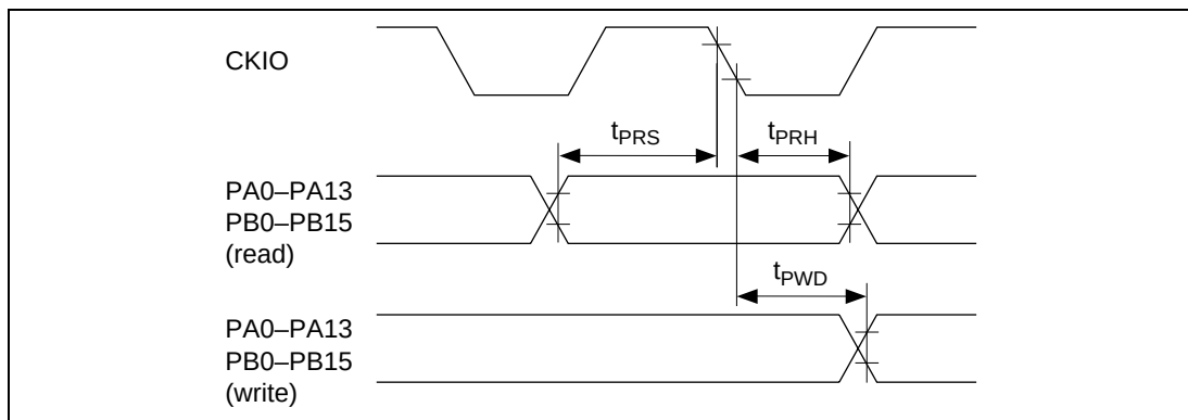
Figure 21.69 I/O Port Input/Output Timing (Except t_{E_{cyc}}:t_{P_{cyc}} = 1:1 )
