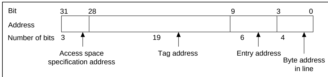
Figure 8.2 Address Configuration
