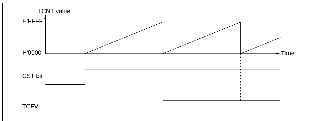
Figure 16.7 Free-Running Counter Operation
