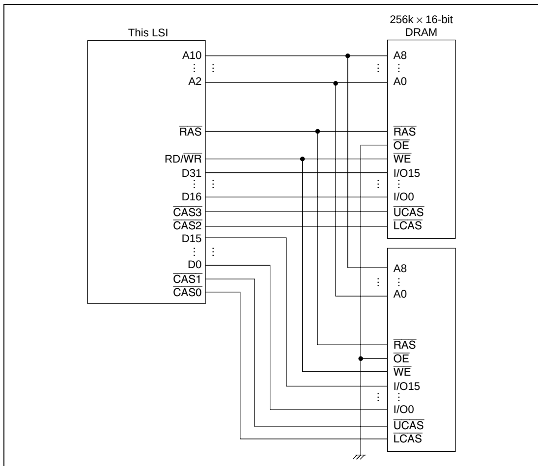
Figure 7.38 Example of DRAM Connection (32-Bit Data Width)
