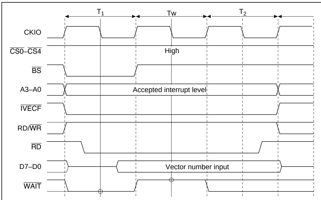
Figure 5.7 External Vector Fetch ( I\phi:E\phi \neq 1:1 ( \overline{\text{WAIT}} Input))
