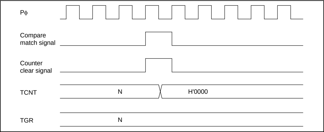
Figure 16.34 Counter Clear Timing (Compare Match)
