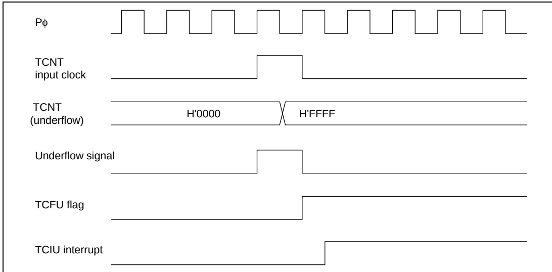
Figure 16.41 TCIU Interrupt Setting Timing
