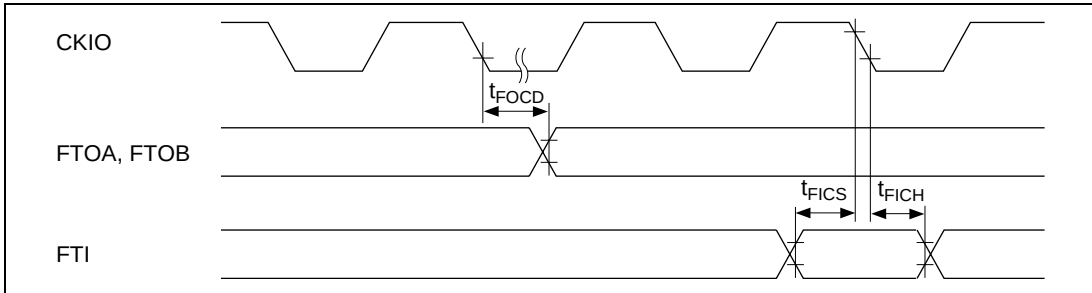
Figure 21.50 FRT Input/Output Timing (Except t_{E_{cyc}}:t_{p_{cyc}} 1:1)
