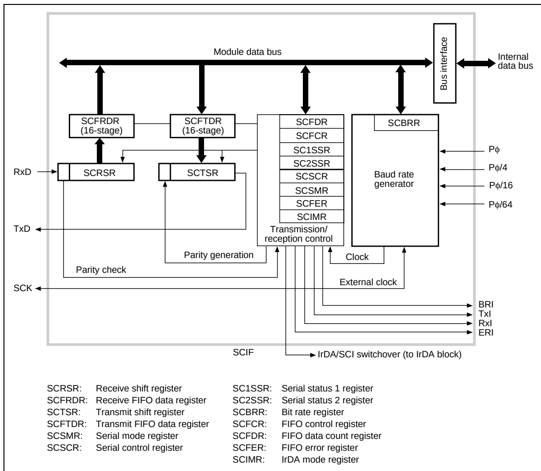
Figure 14.1 Block Diagram of SCIF
