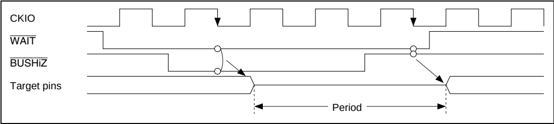
Figure 7.60 BUSHiZ Bus Timing
