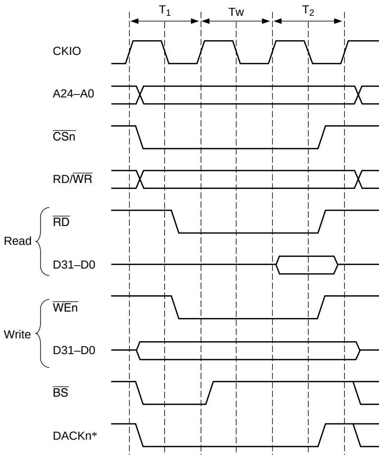
Figure 7.13 Wait Timing of Ordinary Space Access (Software Wait Only)
