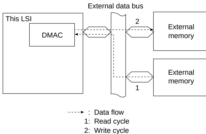
Figure 11.8 Data Flow in Dual Address Mode
