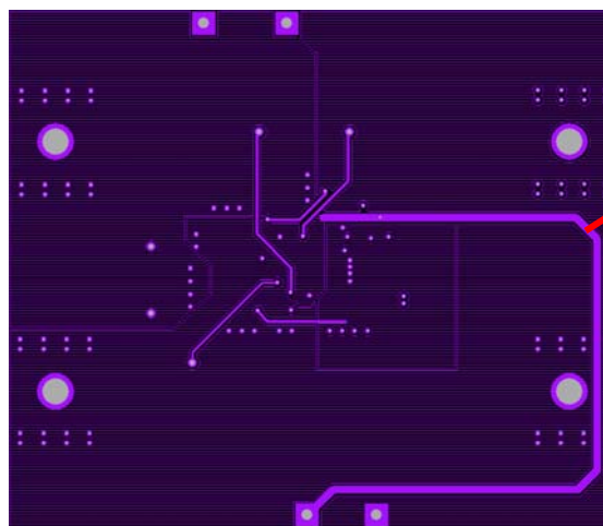
Fig. 26d. IRDC3856 demoboard layout considerations – Mid Layer 2
