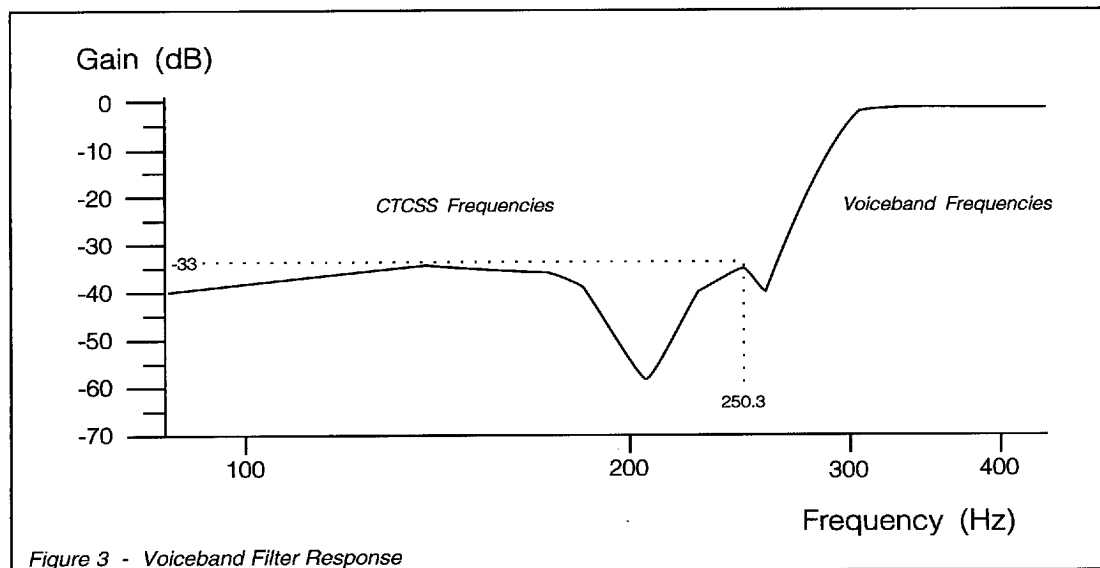
Figure 3 - Voiceband Filter Response
