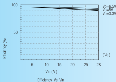
R-74xx Efficiency VS Vin
