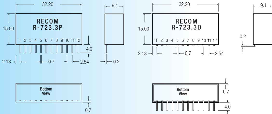
SIP12 PIN Package
