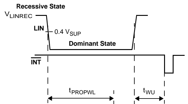
Figure 10. LIN Bus Wake-Up Behavior, Stop Mode
