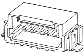
Horizontal Mount
