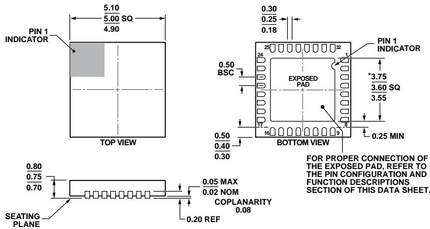
Figure 55. 32-Lead Lead Frame Chip Scale Package [LFCSP_WQ] 5 mm x 5 mm Body, Very Very Thin Quad (CP-32-12) Dimensions shown in millimeters
