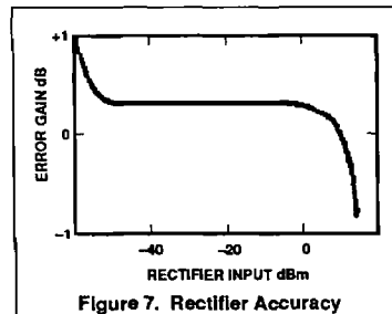
Figure 7. Rectifier Accuracy
