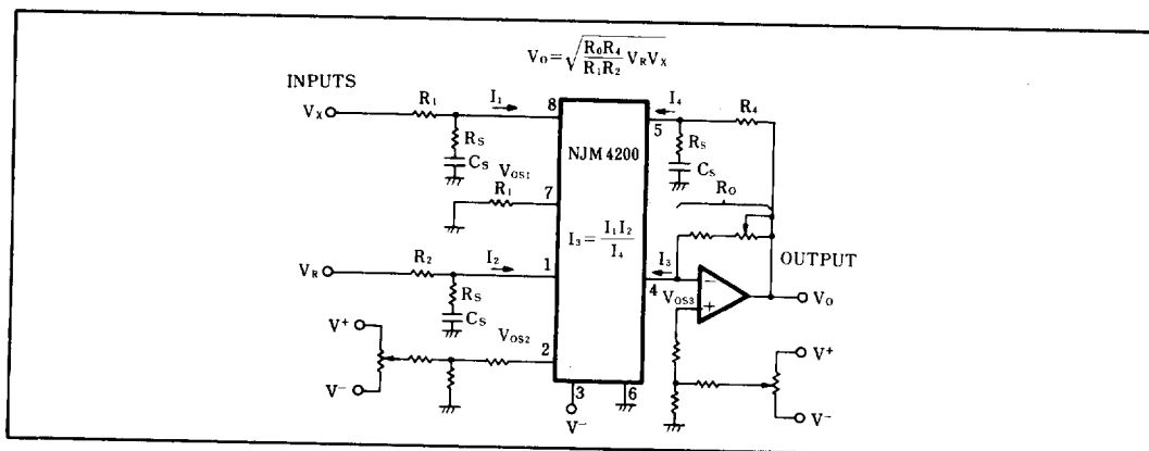
Figure 5. Square-Rooting Circuit
