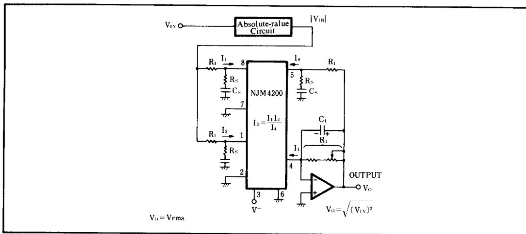
Figure 6. RMS-to-DC Converter
