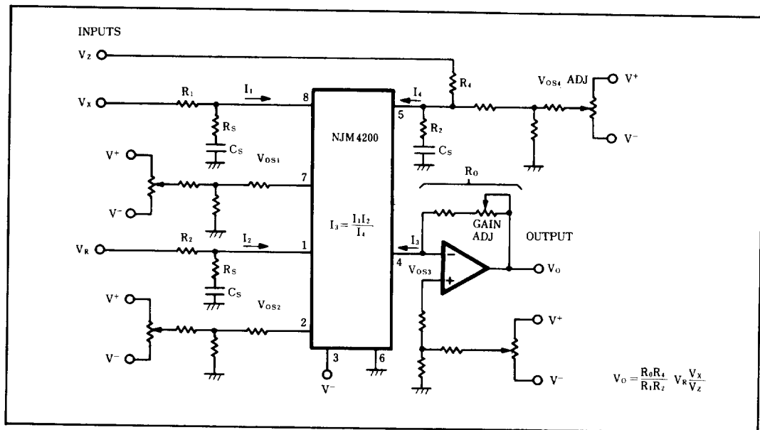
Figure 4. One-Quadrant Divider
