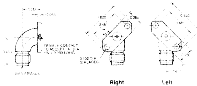
Radius Right Angle Two Hole Flange Female
