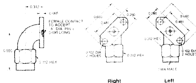
Radius Right Angle Two Hole Flange Mount Male
