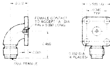
Radius Right Angle Flange Mount Female
