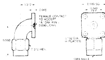
Radius Right Angle Flange Mount Male
