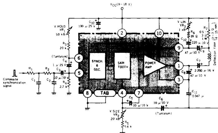
Typical Example of Components Layout with the \mu PC1031H2 on P.C. Board
