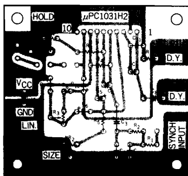
Typical Example of Components Layout with the μPC1031H2 on P.C. Board
