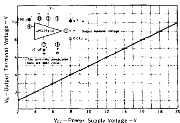
OUTPUT TERMINAL VOLTAGE vs. POWER SUPPLY VOLTAGE
