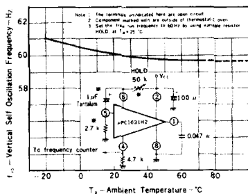
FREE-RUNNING OSCILLATION FREQUENCY vs. AMBIENT TEMPERATURE
