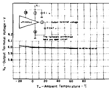
OUTPUT TERMINAL VOLTAGE vs. AMBIENT TEMPERATURE
