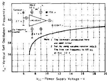
FREE-RUNNING OSCILLATION FREQUENCY vs. POWER SUPPLY VOLTAGE
