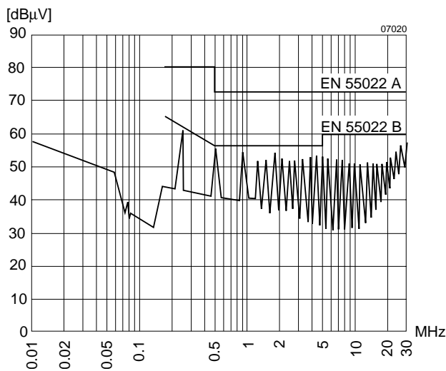
Fig. 16 Typical disturbance voltage (quasi-peak) at the input according to CISPR 11/EN 55011 and CISPR 22/EN 55022, measured at U i,nom and I o,nom . Output leads 0.1 m, twisted. (48 IMS 15-05)
