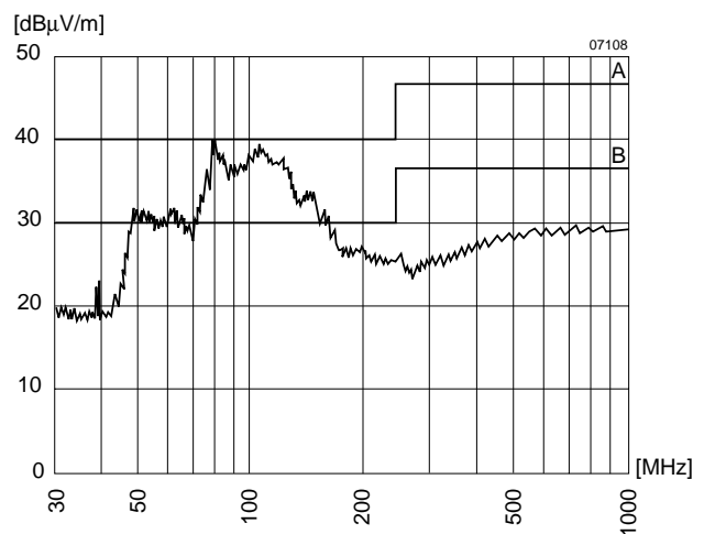
Fig. 17 Typical radio frequency-interference voltage at U i,nom , I o,nom , measured with an antenna (distance 10 m). Output leads 1 m, twisted.
