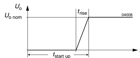
Fig. 6 Converter start-up and rise time.
