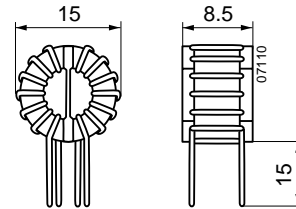
Fig. 19 Choke dimensions (Tokin SC-02-10 GS)
