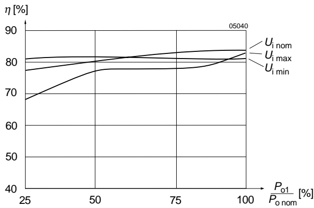
Fig. 12 Efficiency versus input voltage and load. Typical values (48 IMS 15-12-12).
