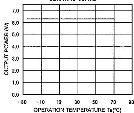
DERATING CURVE
