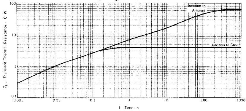
Fig. 13 Z_{th} CHARACTERISTIC
