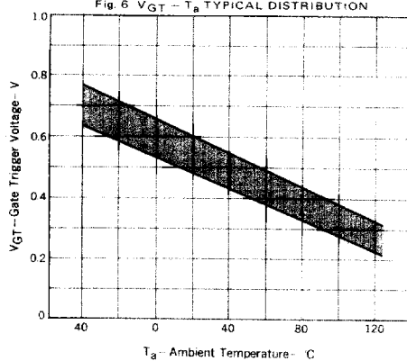
Fig. 6 V_{GT} - T_a TYPICAL DISTRIBUTION
