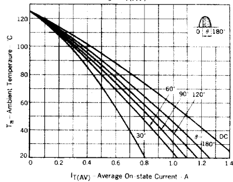
Fig. 12 T_a - I_T(AV) RATING
