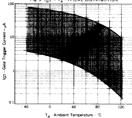
Fig. 5 I_{GT} - T_a TYPICAL DISTRIBUTION
