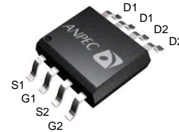
Top View of SOP – 8
