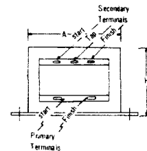
Single 115V
