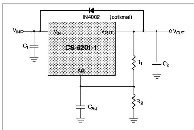
Figure 3. Protection diode for large output capacitors.
