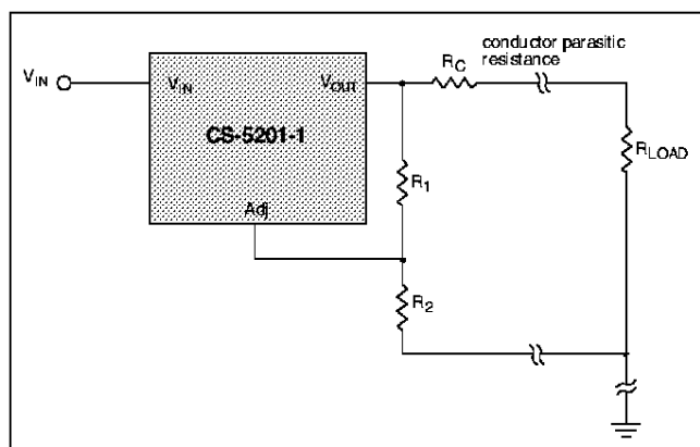
Figure 4. Grounding scheme for the adjustable output regulator to minimize parasitic resistance effects.
