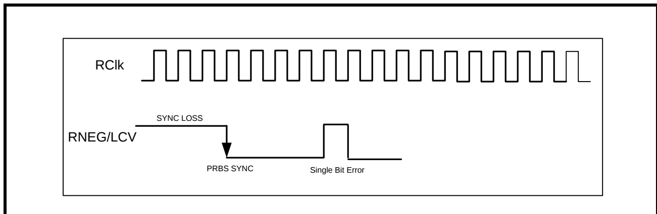
FIGURE 26. PRBS MODE
