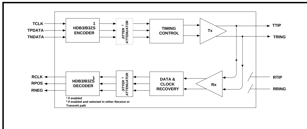
FIGURE 27. ANALOG LOOPBACK
