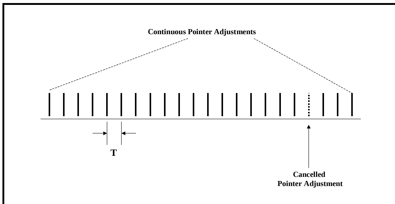
FIGURE 57. ILLUSTRATION OF CONTINUOUS-CANCEL POINTER ADJUSTMENT SCENARIO
