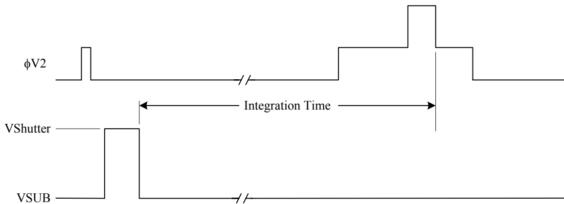
Figure 30: Integration Time Definition
