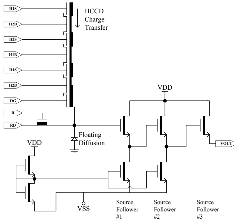
Figure 6: Output Architecture
