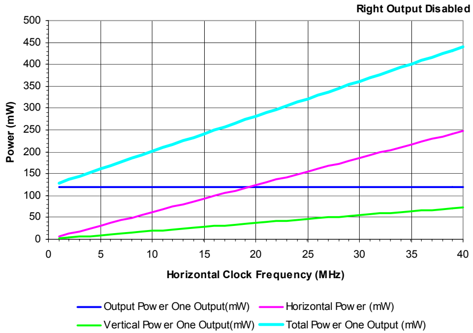
Figure 7: Power
