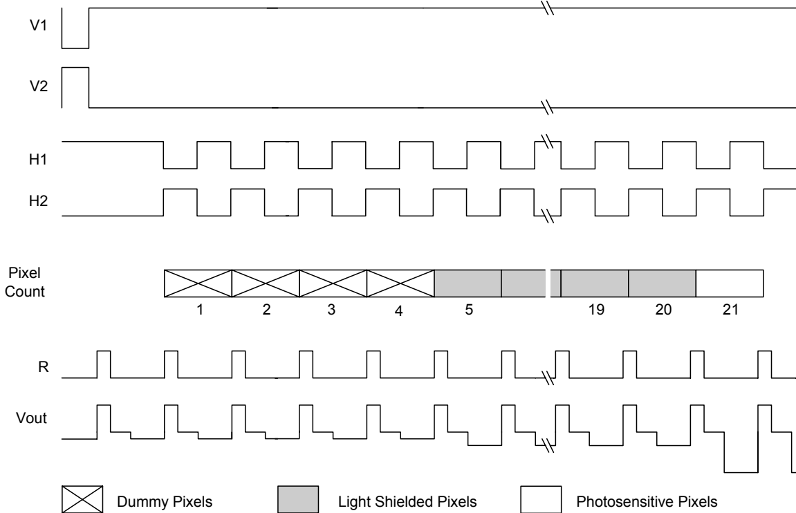
Figure 26: Pixel Timing
