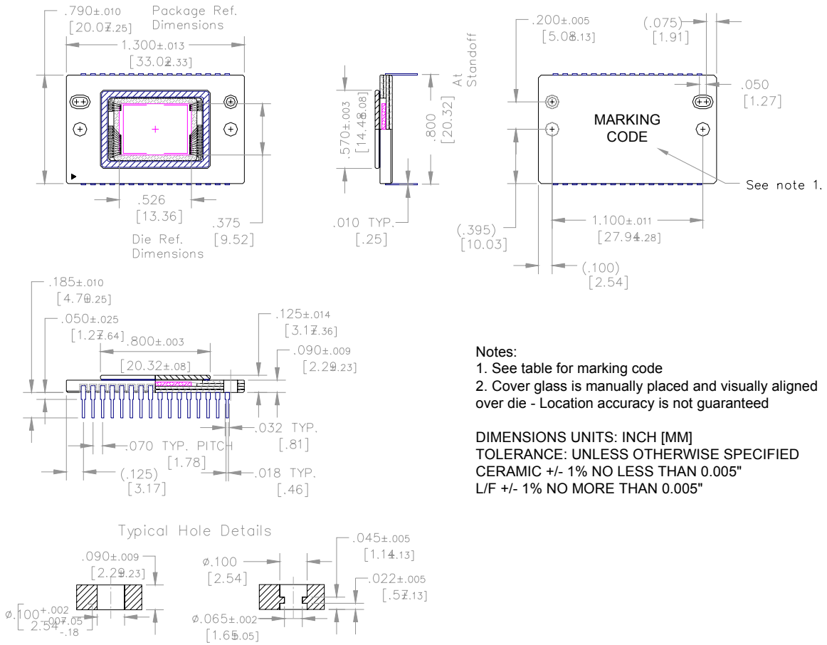
Figure 31: Package Drawing
