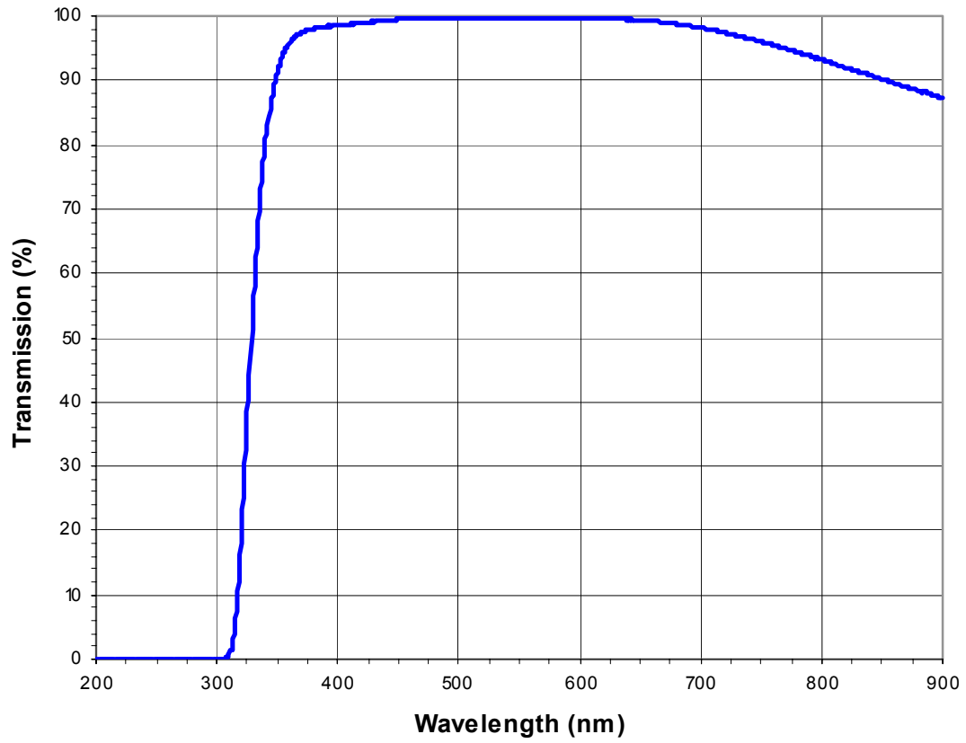
Figure 34: Glass Transmission
