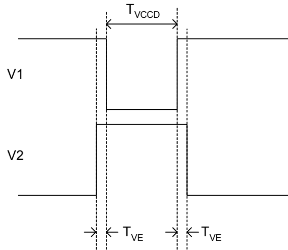
Figure 25: Line Timing Edge Alignment
