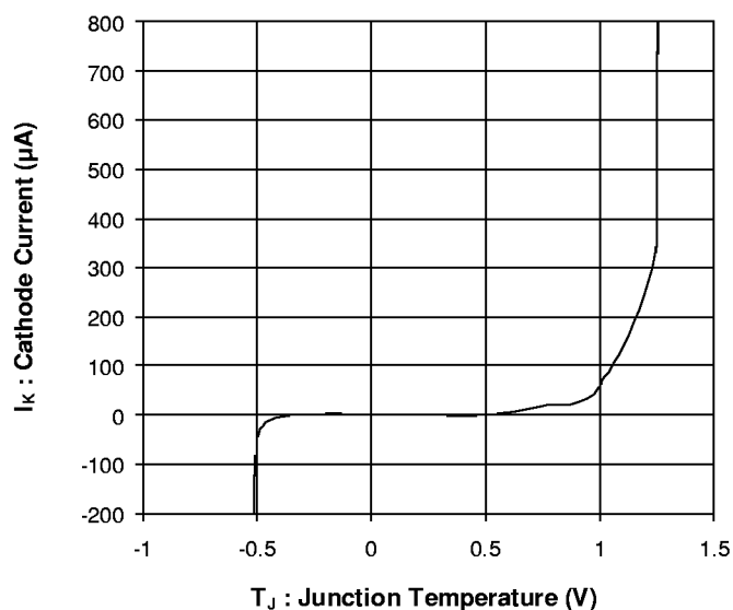
FIGURE 3 — Cathode Current vs. Cathode Voltage
