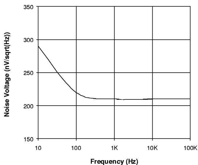
FIGURE 8 — Equivalent Input Noise Voltage vs. Frequency
