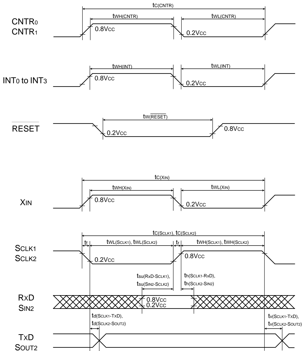
Fig. 60 Timing diagram
