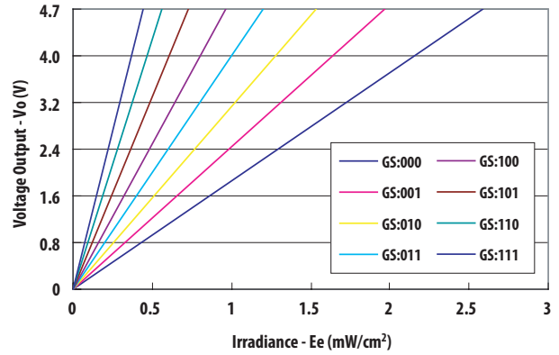
Figure 3. Voltage Output of Blue Channel vs Irradiance ( I_p = 460 nm)
