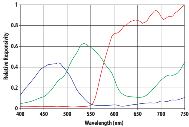
Figure 1. Spectral Responsivity
