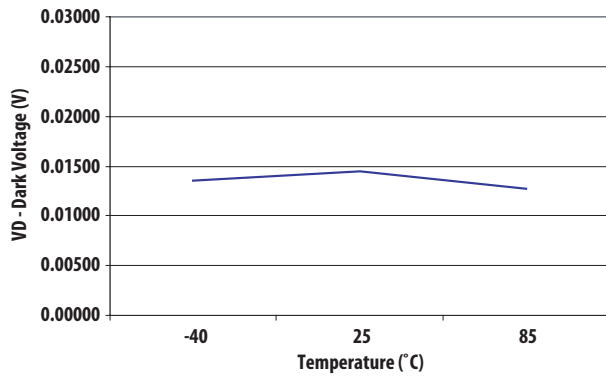
Figure 2. Dark Voltage vs Operating Temperature
