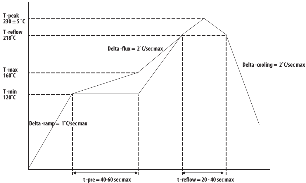
Figure 6. Recommended Reflow Soldering Profile
