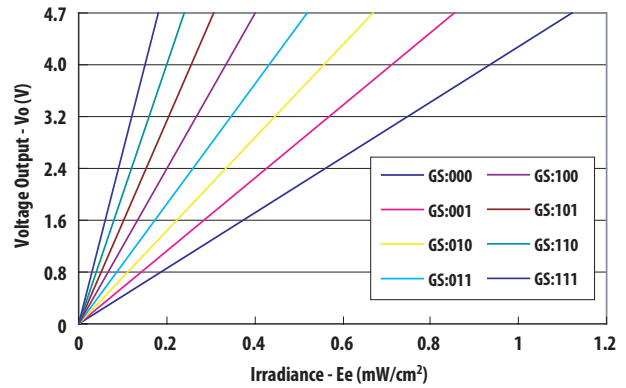
Figure 5. Voltage Output of Red Channel vs Irradiance ( I_p = 645 nm)
