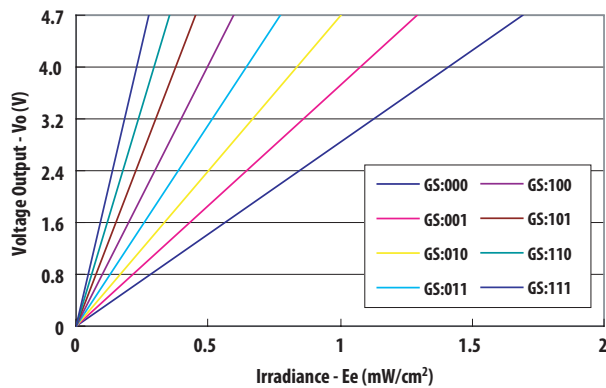
Figure 4. Voltage Output of Green Channel vs Irradiance ( I_p = 542 nm)
