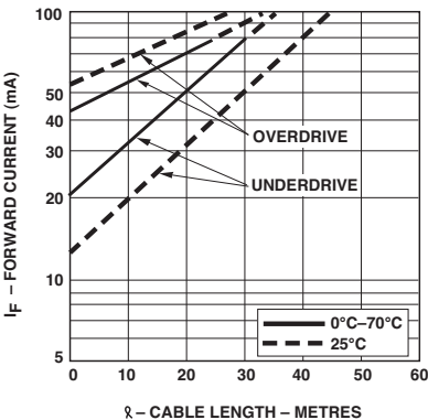
Figure 4. Guaranteed system performance with improved cable (HFBR-15X1Z/25X1Z)
