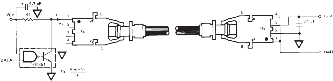
Figure 2. Typical 5 MBd interface circuit
