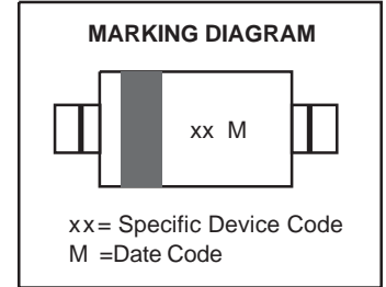
SOD-323
