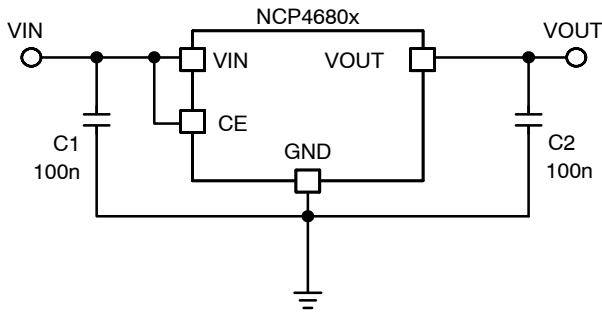
Figure 55. Typical Application Schematic
