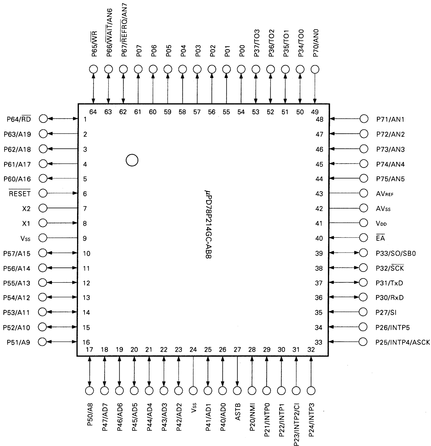
(b) 64-pin plastic QFP
