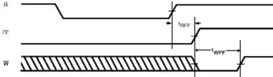
Figure 15. Programmable Half-Full Flag Timing
