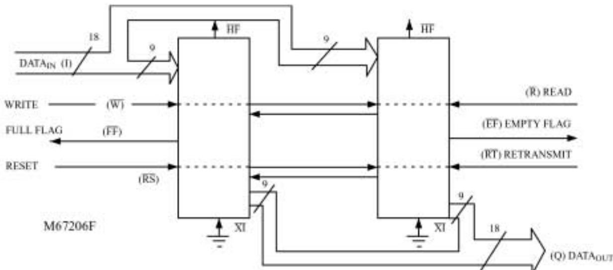
Figure 4. Block Diagram of 16384 X 18 FIFO Memory Used in Width Expansion Mode
