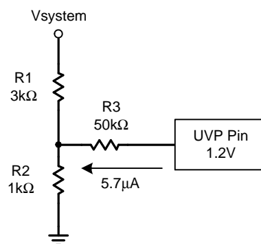
Figure 2. Under-Voltage Protection
