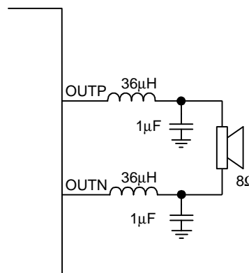
Figure 4. LC output filter for 8Ω speaker
