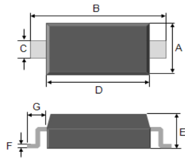
SOD-123
