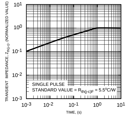
TRANSIENT THERMAL IMPEDANCE CHARACTERISTICS (Each FWD)
