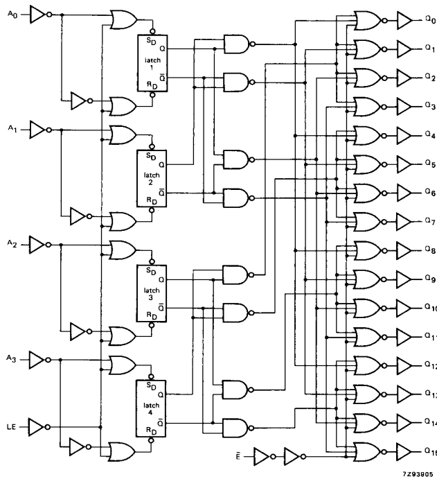
Fig. 5 Logic diagram.
