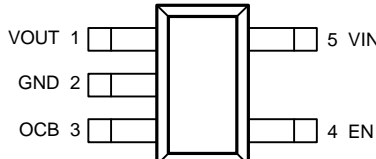
SOT-23-5 APL3518A/C (Top View)
