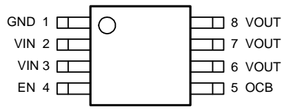
SOP-8/MSOP-8 APL3518A/C (Top View)
