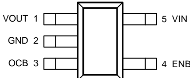
SOT-23-5 APL3518B/D (Top View)
