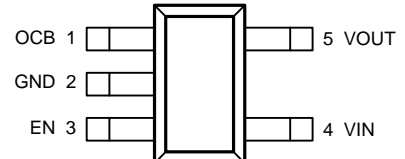
SOT-23-5 APL3519A/C (Top View)
