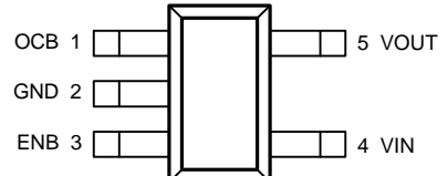
SOT-23-5 APL3519B/D (Top View)
