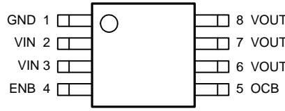
SOP-8/MSOP-8 APL3518B/D (Top View)
