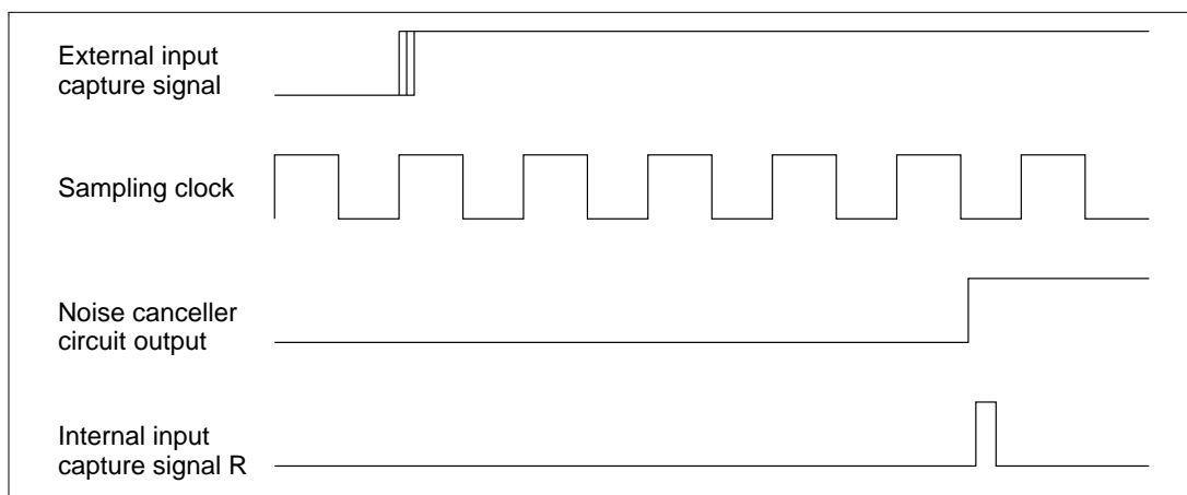
Figure 9.12 Input Capture Signal Timing (Noise Canceller Function Enabled)
