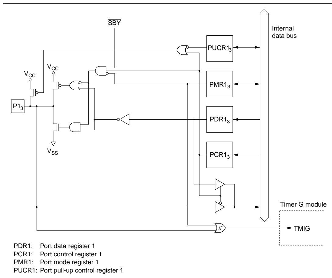
Figure C.1 (c) Port 1 Block Diagram (Pin P1 3 )
