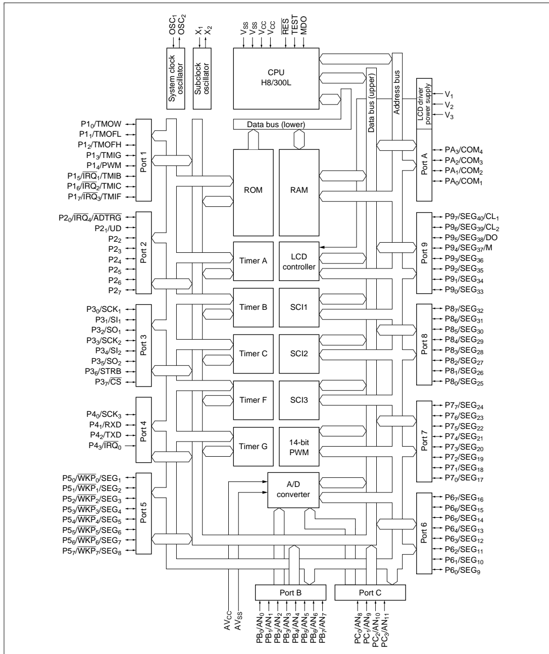
Figure 1.1 Block Diagram
