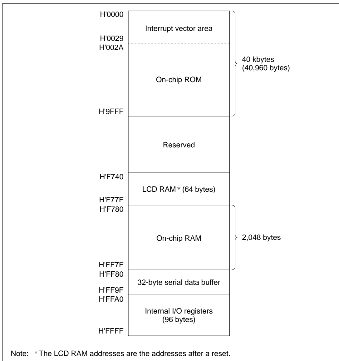
Figure 2.19 H8/3835 Memory Map
