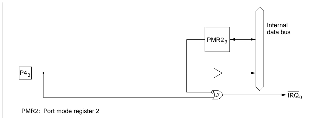
Figure C.4 (a) Port 4 Block Diagram (Pin P4 3 )
