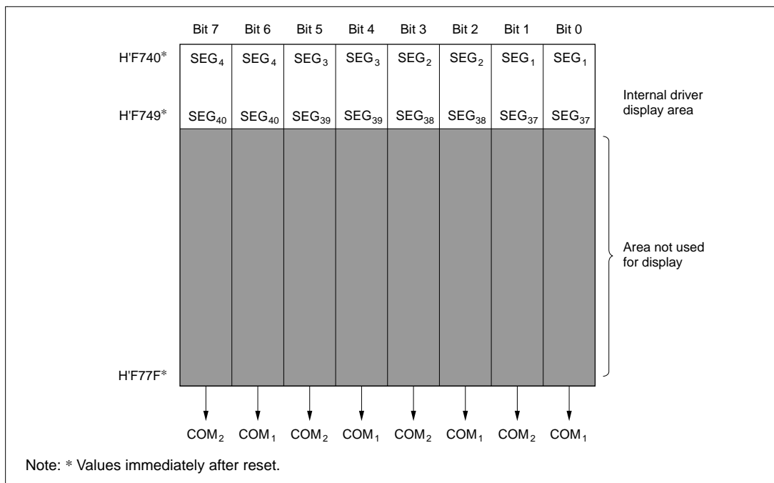
Figure 13.5 LCD RAM Map: No External Segment Expansion (1/2 Duty)
