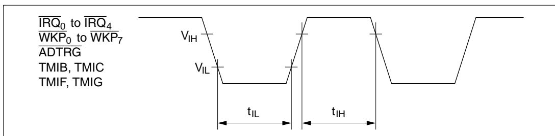
Figure 14.3 Input Timing
