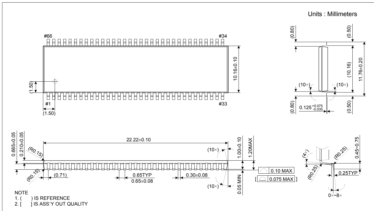
66pin TSOP II 64Mb Package dimension
