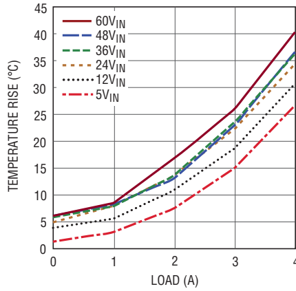
Temperature Rise vs Load, V_{OUT} = 3.3\text{V}
