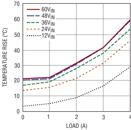
Temperature Rise vs Load, V_{OUT} = 8\text{V}
