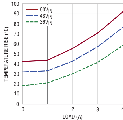
Temperature Rise vs Load, V_{OUT} = 24\text{V}
