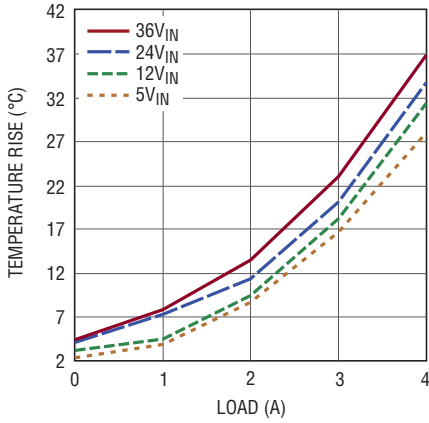
Temperature Rise vs Load, V_{OUT} = 2.5\text{V}
