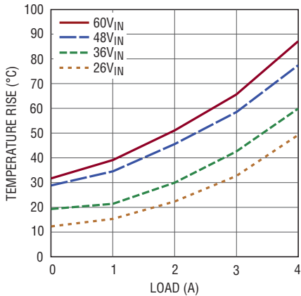
Temperature Rise vs Load, V_{OUT} = 18\text{V}
