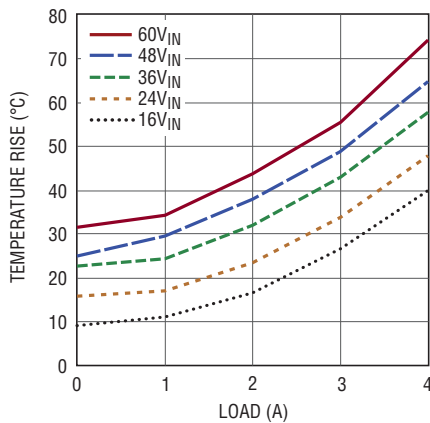
Temperature Rise vs Load, V_{OUT} = 12\text{V}
