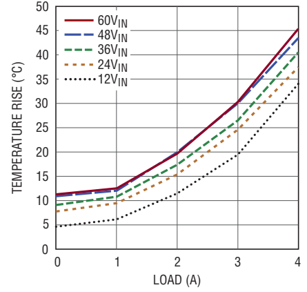
Temperature Rise vs Load, V_{OUT} = 5\text{V}
