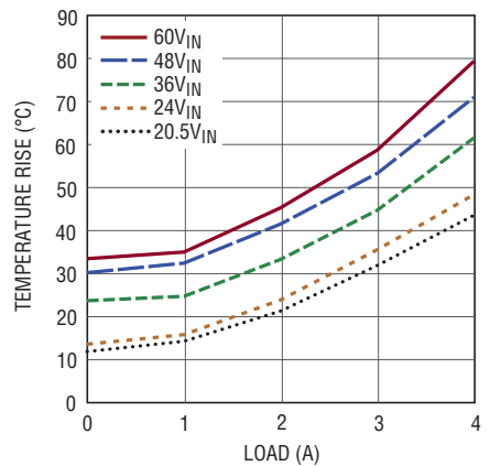
Temperature Rise vs Load, V_{OUT} = 15\text{V}
