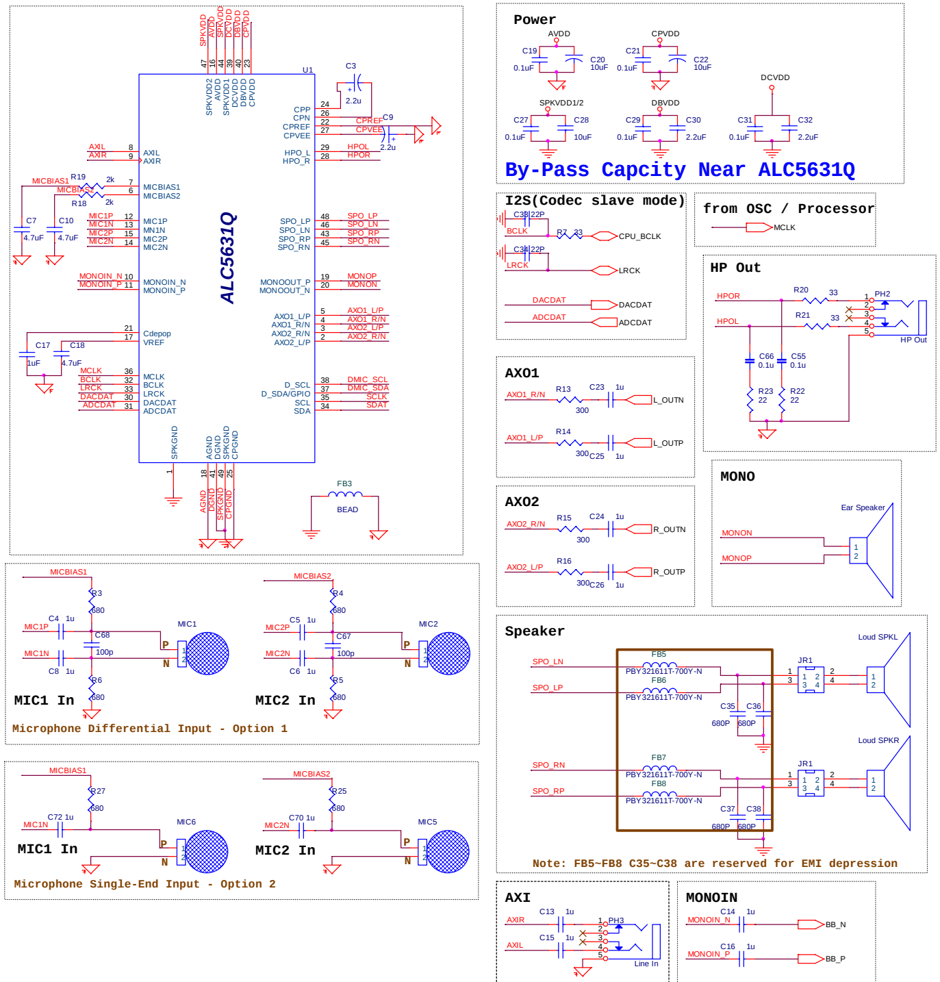
Figure 21. Application Circuit
