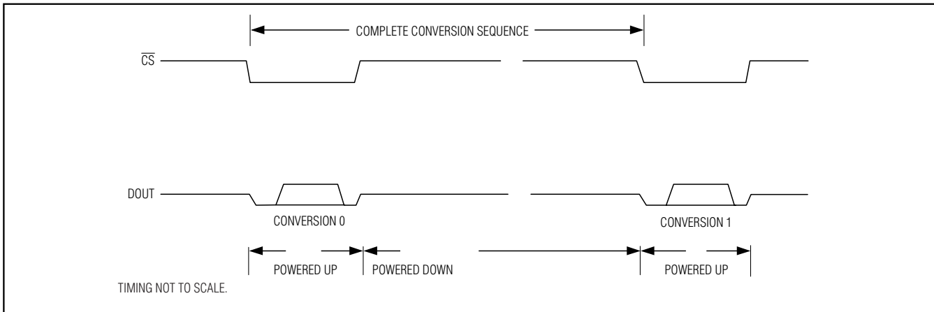
Figure 7. Shutdown Sequence
