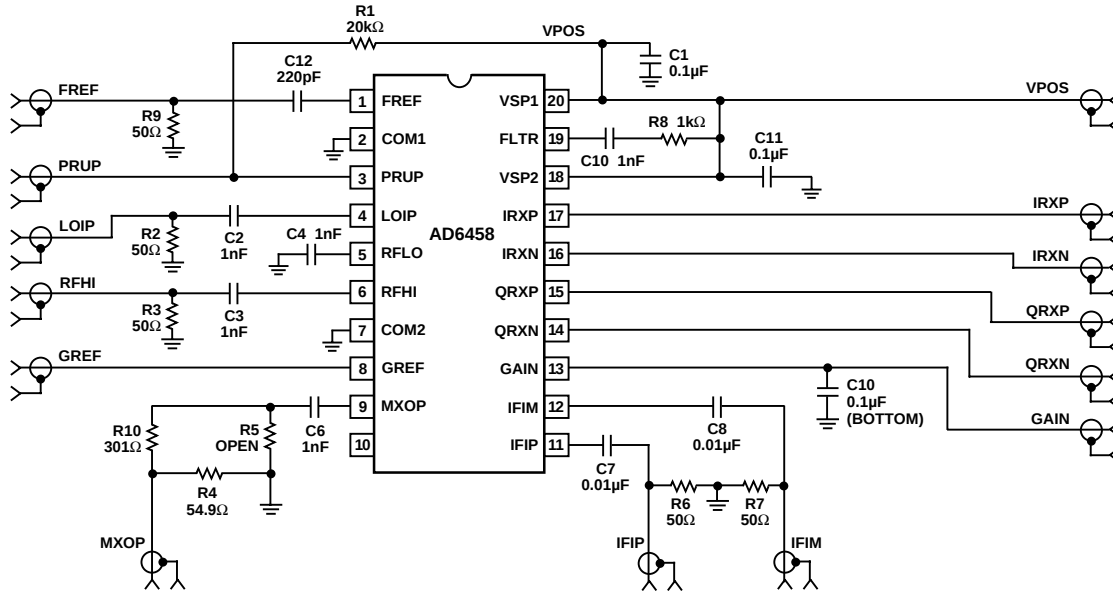
Figure1. Characterization Board
