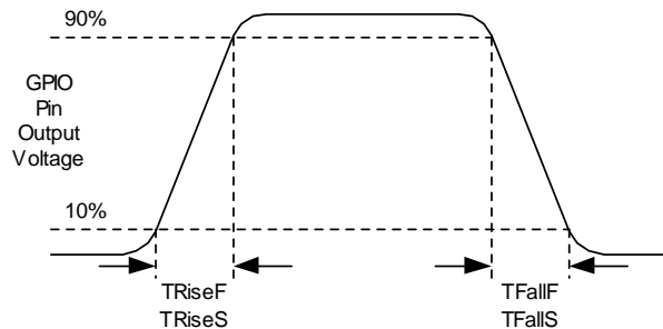
Figure 6. GPIO Timing Diagram
